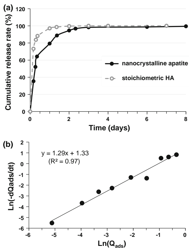
Fig. 8 a Lysozyme release study in HEPES pH 7.3 at 37 °C (immobilization performed in Tris buffer at pH 7.8 on nanocrystalline apatite and on stoichiometric HA), and b linearization data (case of nanocrystalline apatite)
