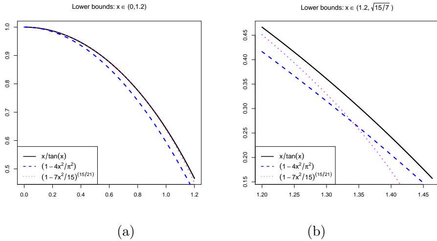
FIGURE 1. Graphs of lower bounds of x/\tan x in (1.2) and (3.11) for (a) x \in (0, 1.2) and (b) x \in (1.2, \sqrt{15/7}) .
