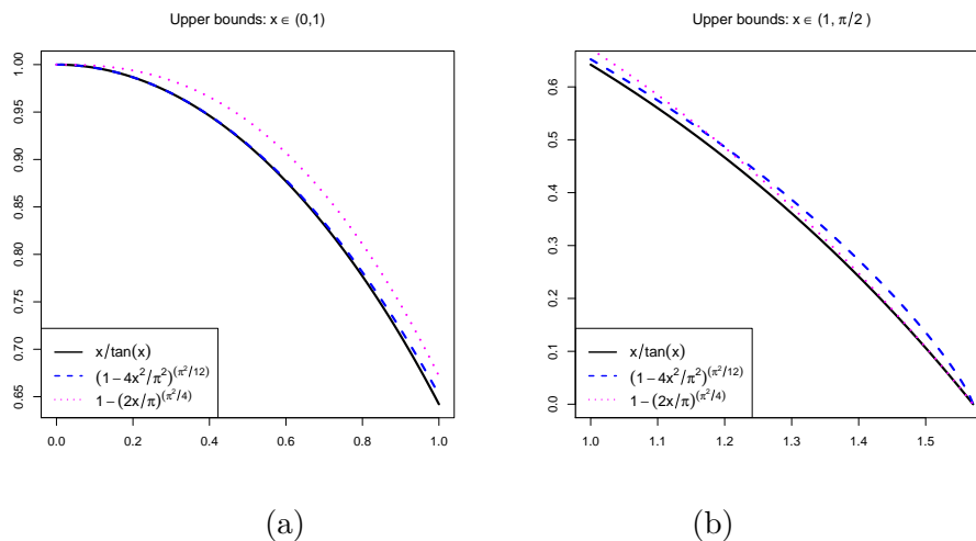
FIGURE 2. Graphs of upper bounds of x/\tan x in (1.2) and (3.3) for (a) x \in (0, 1) and (b) x \in (1, \pi/2) .
