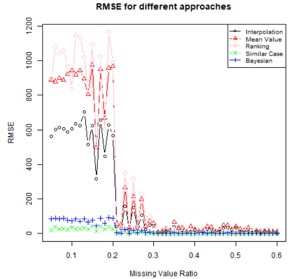
Fig. 4: RMSE for different approaches
