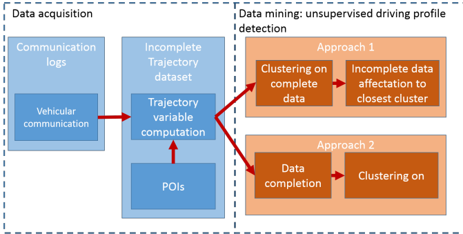
Fig. 1: General pipeline for unsupervised driving profile detection using vehicular communication data
