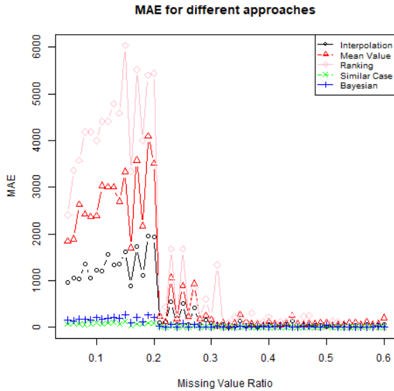
Fig. 5: MAE for different approaches
