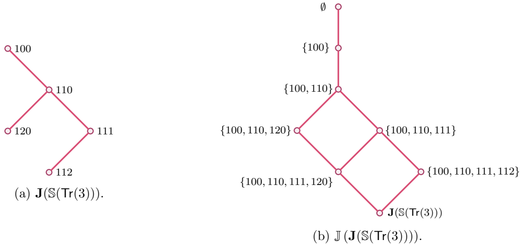
Figure 6: Construction of \mathbb{J}(\mathbb{J}(\mathbb{S}(\text{Tr}(3)))) from the poset \mathbb{J}(\mathbb{S}(\text{Tr}(3))) .
