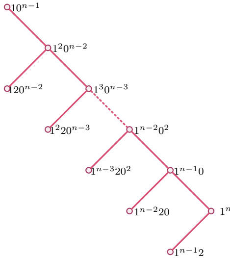
Figure 7: Shape of the poset \mathbf{J}(\mathbb{S}(\text{Tr}(n))) .
