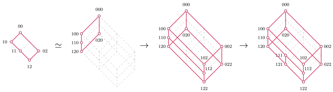
Figure 4: A sequence of interval doubling from \text{Tr}(2) to \text{Tr}(3) .
