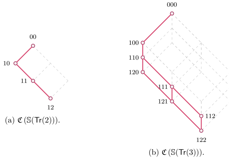
Figure 5: Cubic realizations of some spines of Hochschild posets.
