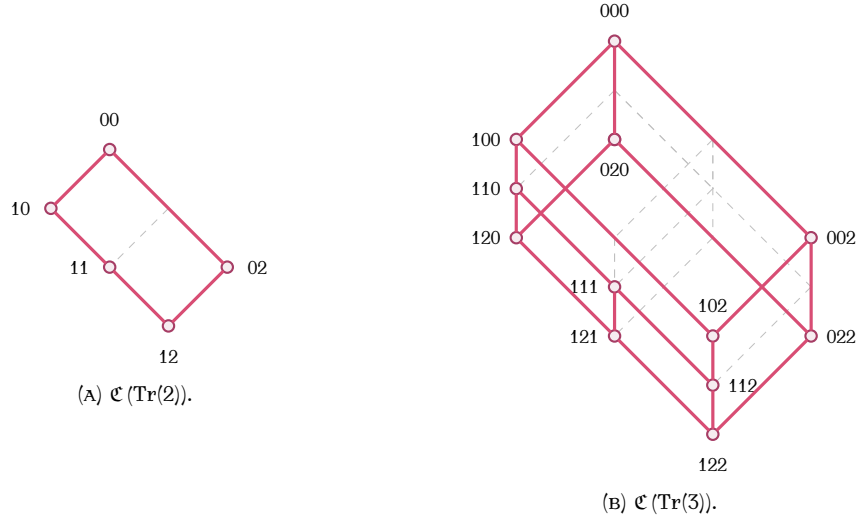
FIGURE 2.4. Cubic realizations of some Hochschild posets.
