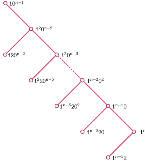
FIGURE 3.3. Shape of the poset \mathbf{J}(\mathbb{S}(\mathrm{Tr}(n))) .
