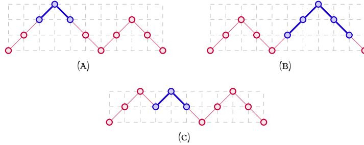
FIGURE 1.2. The three Dyck paths covering the Dyck path 1100101100 for the dexter order.
