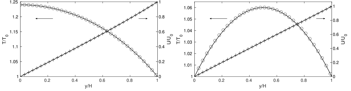
Figure 4: Temperature and velocity profiles of the thermal couette flow for \gamma = 7/5 , \text{Pr} = 0.71 and \text{Ma} = 1.3 . The solid lines \text{—} correspond to analytical results; the numerical results + and o correspond respectively to the velocity profiles U/U_0 and the temperature profiles T/T_0 . Boundary conditions: isothermal top wall and adiabatic bottom wall (left), isothermal walls (right).
