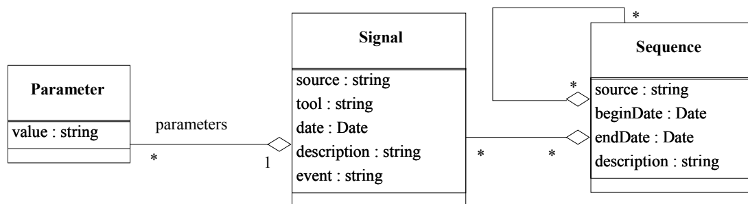
Figure 5. UML model
