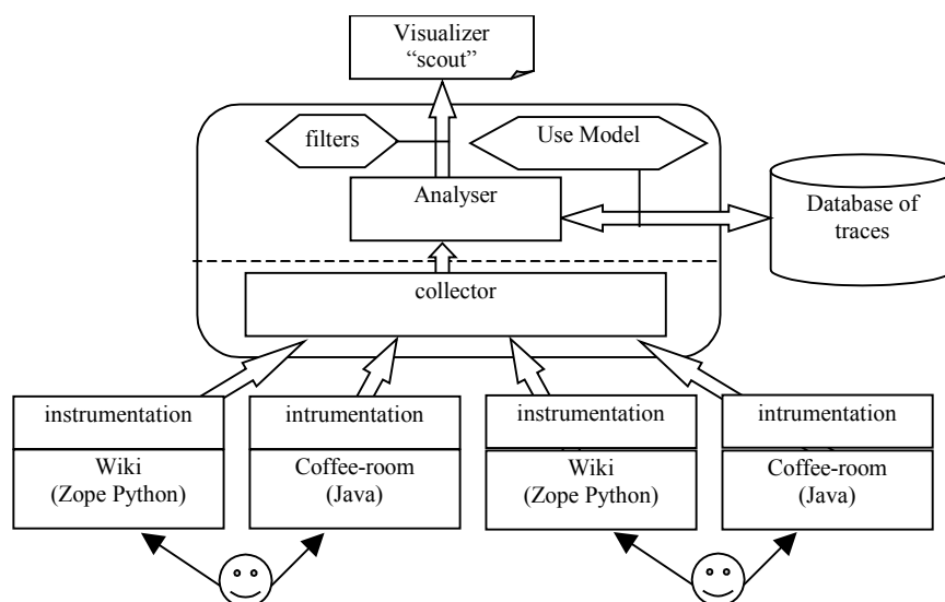
Figure 4. Architecture of an observation station
