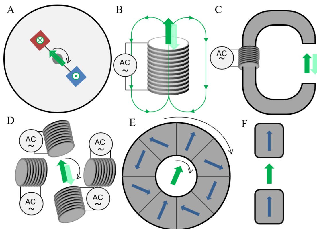
Fig. 3. Simplified diagrams of the mainly used magnetic field application devices. a) Magnetic stirrer composed of two magnets at the end of a rotating rod (top view). b) A coil powered by an alternating current that creates an alternating magnetic field inside or above the coil. The arrows in loops represent the magnetic flux line. c) Ferrite core surrounded by a copper coil through which a sinusoidal alternating current flows. d) System composed of 4 coils powered by an alternating sinusoidal current. The amplitude, phase shift and frequency of the applied current can be chosen to create an alternating or rotating field in the center of the 4 coils. e) Halbach cylinder composed in this example of 8 permanent magnets creating an homogeneous field in the hollow of the cylinder. The rotating field is obtained by rotating the cylinder. f) System composed of two magnets allowing to create a relatively homogeneous constant field.
