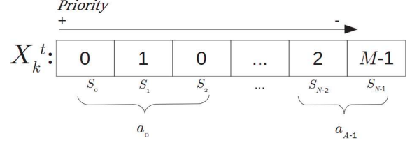
Fig. 1: Position of the k^{th} particle after t iterations.
