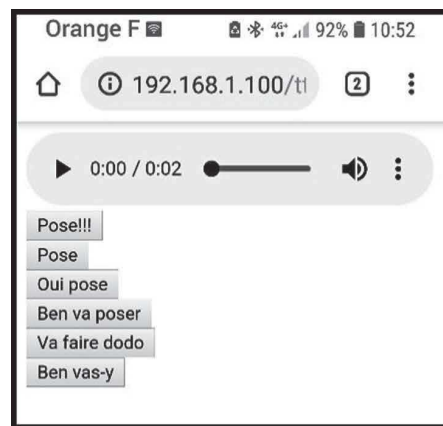
Fig. 3. VCT interface.
