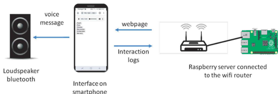
Fig. 2. VCT infrastructure.
