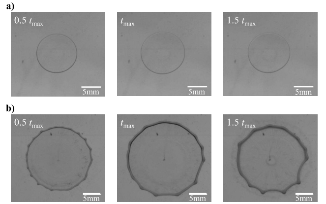
FIG. 4. Snapshots taken at different times, as indicated, during the expansion and retraction of the sheet for (a) a Newtonian silicon oil with shear viscosity \eta_0 = 658 mPa.s ; maximum expansion reached at time t_{max} = 5.22 ms and (b) a PEO solution with C = 0.6\text{wt}\% and \eta_0 = 628 mPa.; maximum expansion reached at time t_{max} = 5.02 ms. The bar sets the scale.
