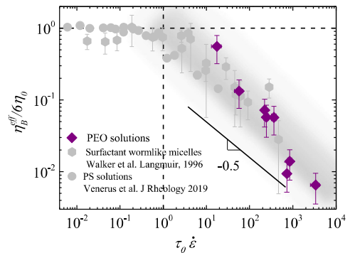
FIG. 9. Effective biaxial extensional viscosity of PEO solutions, extracted from the manual shift of the data in Fig.7, normalized by the plateau biaxial extensional viscosity as a function of the Weissenberg number, plotted together with literature data as indicated in the legend. A unique master biaxial extensional flow curve is obtained with a thinning exponent of -0.5 in agreement with theoretical predictions (see text). The grey zone highlights the -0.5 slope.
