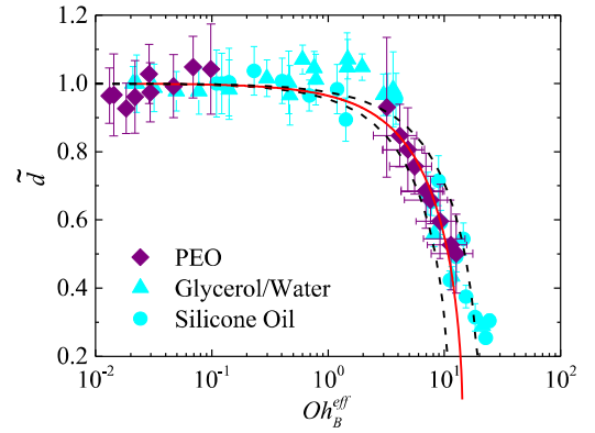
FIG. 7. Normalized maximum expansion factor as a function of the effective biaxial extensional Ohnesorge number for polymer solutions and for the two classes of Newtonian samples. The thin continuous line is the best fit with Eq. 11, and the dashed lines are used to evaluate error bars on the fit parameter.
