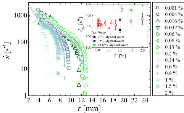
FIG. 8. Evolution of the expansion strain rate as a function of the sheet radius during its expansion for aqueous PEO solutions at different concentrations, as indicated in the legend. Inset: Average strain rate calculated according to Eq. 4 as a function of concentration. Error bars represent the standard deviation from three different experiments.
