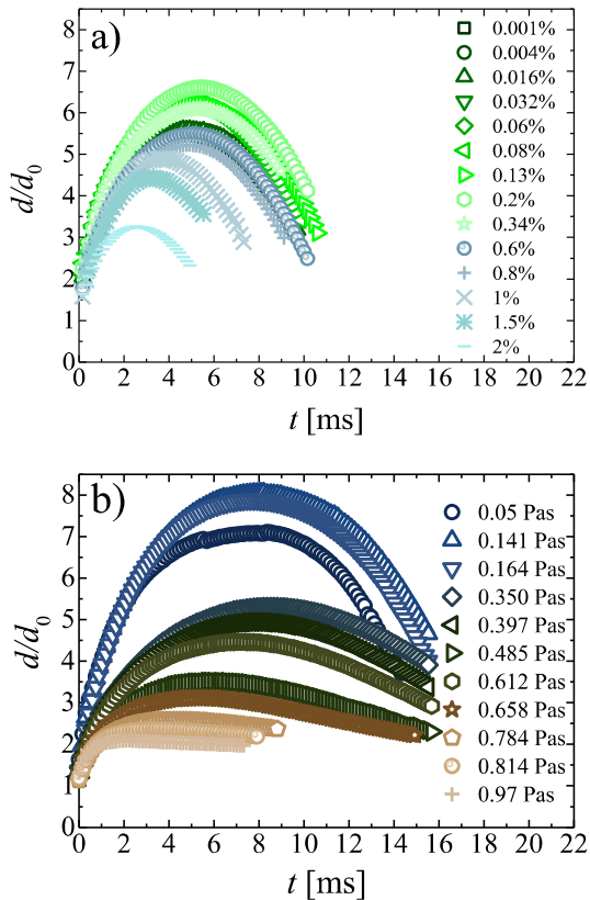
FIG. 5. Time evolution of the sheet diameter normalized by the initial drop diameter for (a) PEO solutions with different concentrations and (b) silicon oils with different shear viscosities, as indicated in the legends. The origin of the time is taken at the drop impact.
