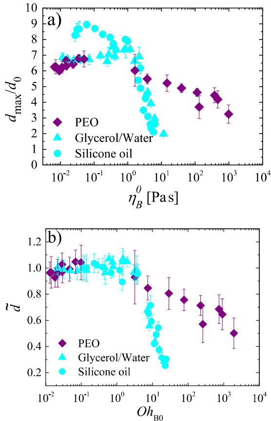
FIG. 6. a) Maximum diameter of the sheet normalized by the initial drop diameter as a function of the biaxial extensional viscosity, and b) Normalized maximum expansion factor as a function of the biaxial extensional Ohnesorge number, for PEO solutions and for Newtonian liquids.
