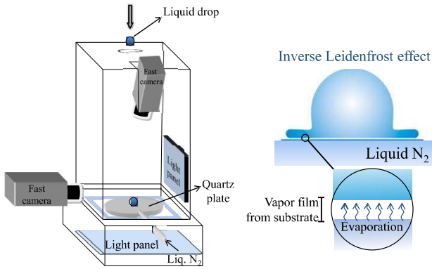
FIG. 1. Left: Schematic illustration of the impact experiments setup showing a drop falling on a liquid nitrogen thin layer. The expansion event is recorded using two fast cameras allowing concomitant top and side visualizations. Right: adapted from [34], schematic of the inverse Leidenfrost effect at the origin of the shear free expansion.
