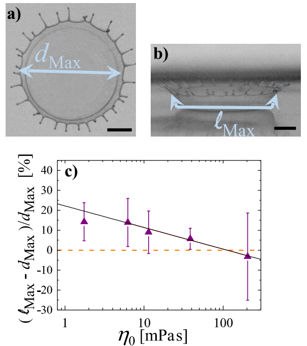
FIG. 2. (a): Top view and (b): side view snapshots of the maximum expansion of a low viscous Newtonian sample (22 wt% Glycerol/water mixture), revealing that the effective diameter d_{\text{Max}} from the top view underestimates the maximum expansion of the sheet \ell_{\text{Max}} . (c): Relative side view correction effect (in %) as a function of shear viscosity of Newtonian glycerol/water. The line is an empirical fit of the data points (symbols).
