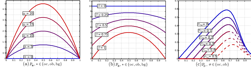
Fig. 3 (a) Binarising penalty in the amplitude strategy, BiP \alpha , with \alpha \in [0, 20] and \beta = 1 . (b) Binarising penalty in the frequency strategy, BiP \beta , with \alpha = 20 and \beta \in [0, 1] . (c) Thinning penalty, TiP, for p_{bg} \in [0, 0.5] . The dashed parts are not applicable, with p_{bg} + p_{\#} > 1 .
