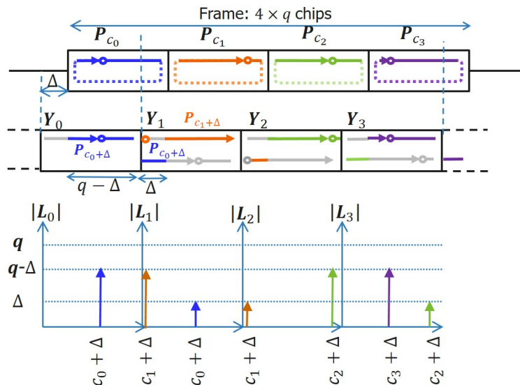
Fig. 3: Illustration of frame detection principle
