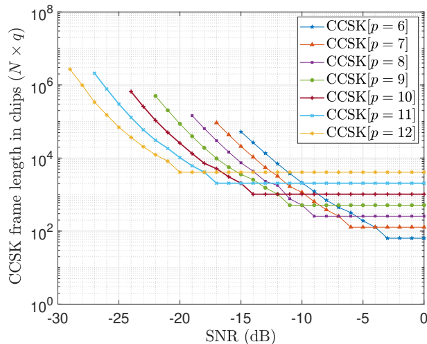
Fig. 8: Minimum CCSK frame length in chips, needed for \mathcal{P}_{\text{md}} \leq 10^{-4} and \mathcal{P}_{\text{fa}} \leq 10^{-6} , for different p values in an ideally synchronized channel.
