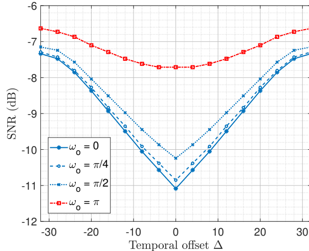
Fig. 7: Minimum SNR required as function of different \Delta and \omega_0 values, for defined probabilities ( \mathcal{P}_{fa} = 10^{-6} and \mathcal{P}_{md} = 10^{-4} ), in a CCSK frame of q = 64 , m = 120 bits and R_c = 1/3 .
