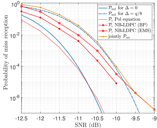
Fig. 9: Joint frame error rates due to \mathcal{P}_e , \mathcal{P}_{\text{md}} and to \mathcal{P}_{\text{fa}} = 10^{-6} for m = 120 , R_c = 1/3 and \text{GF}(2^6) .
