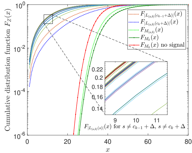
Fig. 4: Illustration of different CDF equations for a given GF(64) received block \mathbf{Y}_k at SNR=-7 dB, \Delta = 24 chips and \omega_o = \pi/4 .
