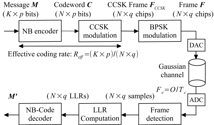
Fig. 2: CCSK-based System Model
