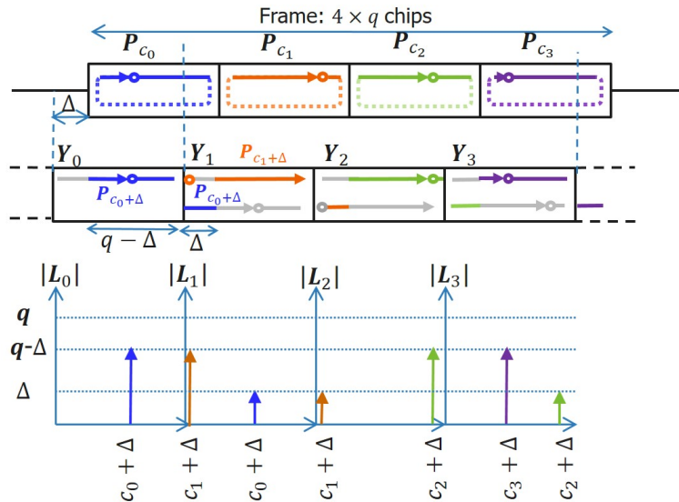
Fig. 3: Illustration of frame detection principle
