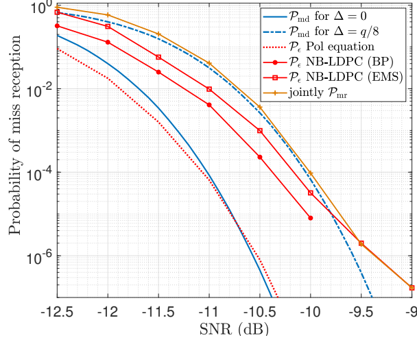
Fig. 9: Joint frame error rates due to \mathcal{P}_e , \mathcal{P}_{md} and to \mathcal{P}_{fa} = 10^{-6} for m = 120 , R_c = 1/3 and \text{GF}(2^6) .
