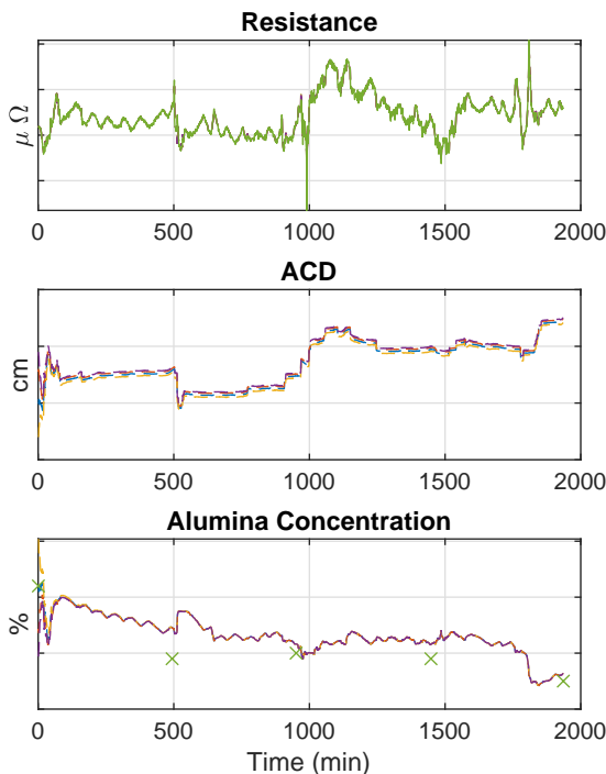
Fig. 6. States Estimations - Data Set 2
