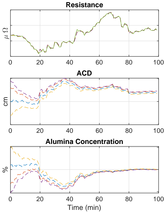
Fig. 5. States Estimations - Data Set 1
