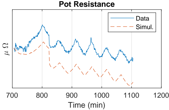
Fig. 4. Resistance Model Validation
