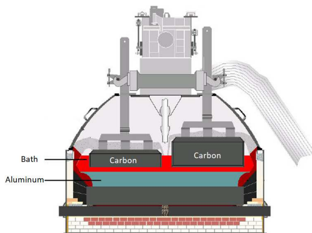
Fig. 1. Pot Schematic View
