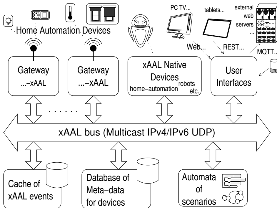
Figure 1. Functional architecture of xAAL.
