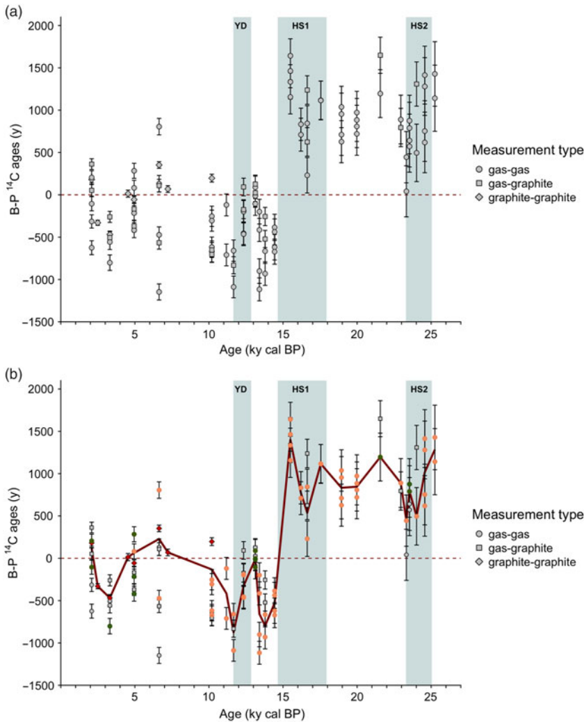
Figure 5 SU90-08 B-P ^{14}\text{C} ages time series: (a) Raw B-P ^{14}\text{C} ages obtained from all pairs of measurements with the available dataset. The symbol type indicates the measurement type: gas vs gas measurements are represented by circles, gas vs. graphite by squares and graphite vs graphite by diamonds. (b) Screened B-P ^{14}\text{C} ages time series. The red symbols correspond to graphite vs. graphite B-P pairs. The orange symbols correspond to the data that passed the leaching control (see Figure S5). The green symbols represent pairs for which one graphite measurements agrees with one benthic or planktonic gas measurement within 2\sigma uncertainty. The bold red line connects the average screened data (i.e. colored symbols).
