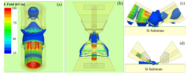
Fig. 8. E-field distribution in the transistor-open at 220 GHz using the probes designed for 140 GHz - 220 GHz ((a) and (c)) and 325 GHz - 500 GHz ((b) and (d)), where (a)-(b)= top view, (c)-(d)= side view.
