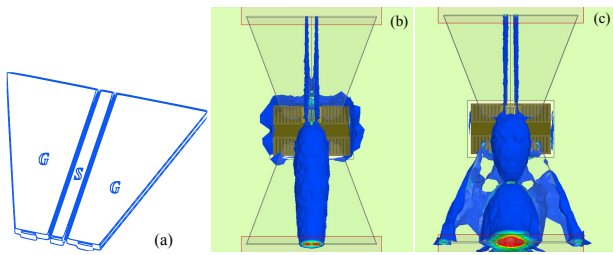
Fig. 10. E-field distribution in the transistor-open using the probe model shown at (a) 110 GHz in panel (b) and 220 GHz in panel (c). In the probe shown in (a), the signal trace width is 25\mu\text{m} , the ground trace minimum width is 63\mu\text{m} and the metal thickness is 8.66\mu\text{m} .
