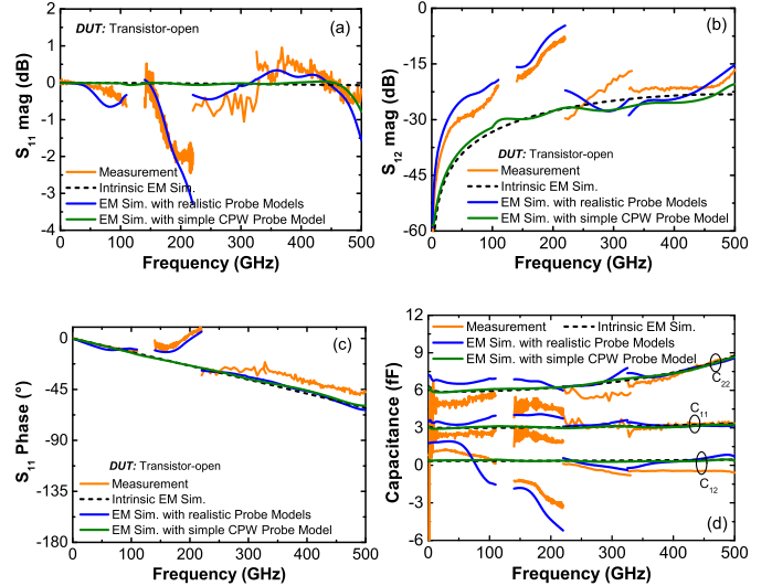
Fig. 5. S-parameter and capacitance measurements along with the EM simulation of the transistor-open up to 500 GHz. The solid blue and green lines shows predictions of RF probe models shown in Fig. 2 and Fig. 10, respectively.
