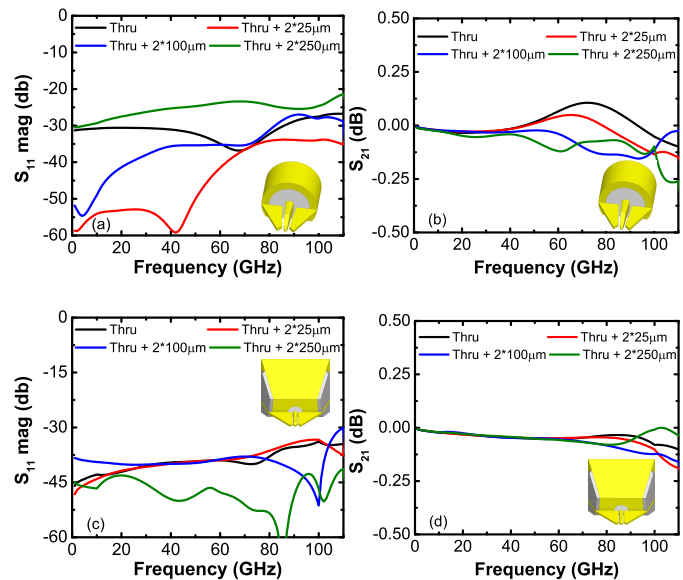
Fig. 12. S-parameter (magnitude of S_{11} and S_{21} ) of a 120\mu\text{m} long line using a thru with different access line lengths in the on-wafer TRL calibration. for all the cases, the reference plane is set at the same position as for the original thru. Results in panel (a) and (b) are obtained from using a RF probe corresponding to 1 GHz - 110 GHz while results of (c) and (d) are obtained using the probe corresponding to the 325 GHz - 500 GHz frequency range.
