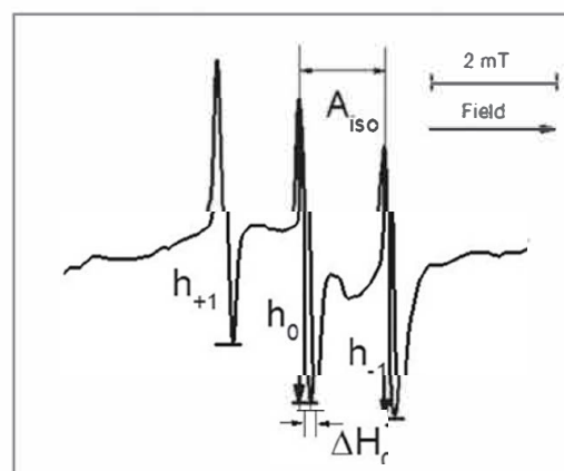
Figure 4. EPR spectrum of the probe in physiological solution 24 h after the introduction of nanohorns.
