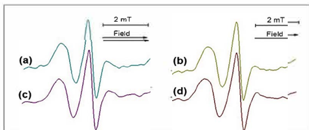
Figure 7. EPR spectra of the probe in the erythrocyte suspension after 10 min (a, b) and 1 h (c, d) after introduction of the inCNH (a, c) and oxCHN (b, d).
