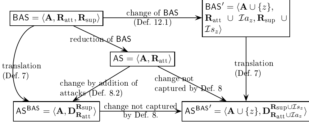
Figure 2: Links between the different systems
