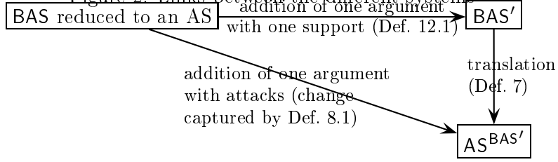
Figure 3: Links between systems if there is no support in BAS
