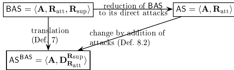
Figure 1: The translation of \text{BAS} into \text{AS}^{\text{BAS}} is an update
