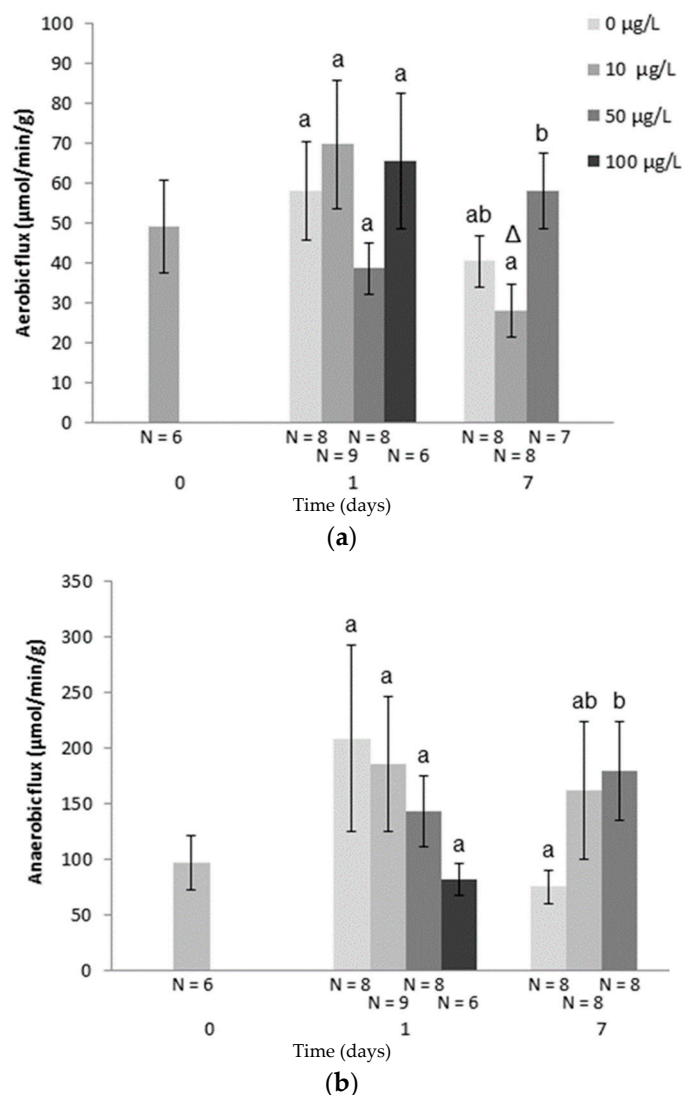
Figure 1. (a) Aerobic flux ( \mu\text{mol/min/g} ) and (b) anaerobic flux ( \mu\text{mol/min/g} ) in white muscle of juvenile roach during Cu exposure. Bars represent S.E. Different letters indicate significant differences for the same time point. \Delta indicates significant differences for the same concentration among individual samples at T1 and T7.
