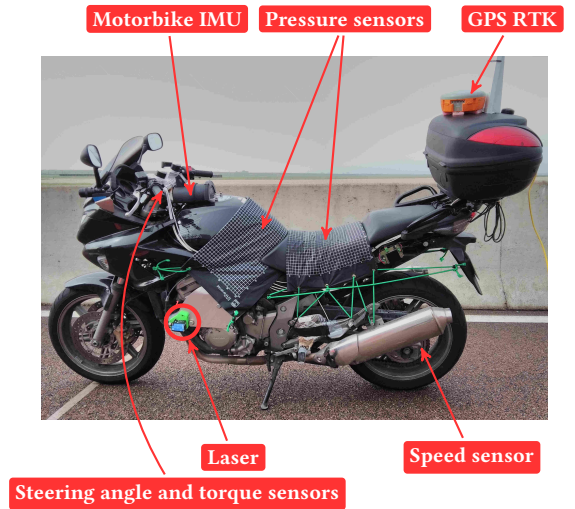
Fig. 4: The instrumented motorbike (VIROLO++ project)
