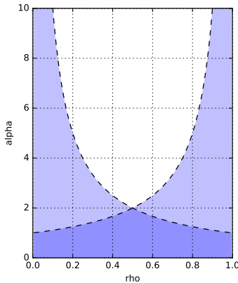
Figure 6: Admissible values of the hyperparameters in the MAP algorithm presented in Section 3.5. Admissible values are in white.
