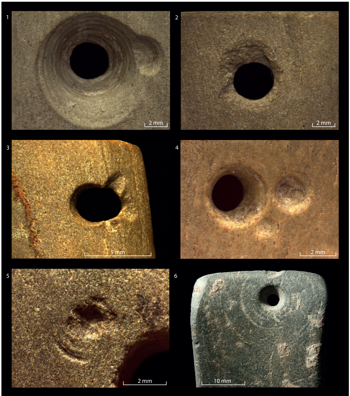
Fig. 10. Details of various bracer perforations: (1–2) abandoned perforation and completed conical perforation on inner face and chipped outline of perforation on outer face, Hoštice I, grave 915/02, Moravia (CZ122; MV, no. A84792); (3) biconical perforation with edge partly chipped during drilling, Hulín 2 'Pravčice', grave H59, Moravia (CZ091; ACO, no. 04/2007–861-3); (4) perforation and two abandoned perforations, Radovesice-Bílina III, grave 53/80-I, Bohemia (CZ053; RMT, no. 44524); (5) abandoned perforation with drilling striations, Radovesice-Bílina III, grave 53/80-II, Bohemia (CZ054; RMT, no. 44526); (6) large-diameter drilling striations, Třebovle, Bohemia (CZ016; RMK, no. 9127) (photos: C. Nicolas).
