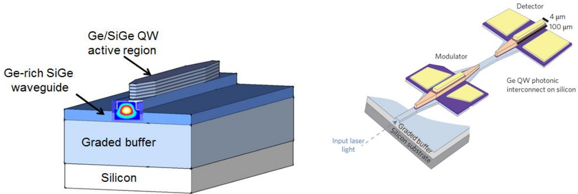
Fig. 3. Integration of Ge/SiGe QW devices with Ge-rich SiGe waveguide on graded SiGe buffer. (a) SiGe waveguides coupled with the QW active region ; (b) : optical link based on a modulator, a waveguide and a photodetector
