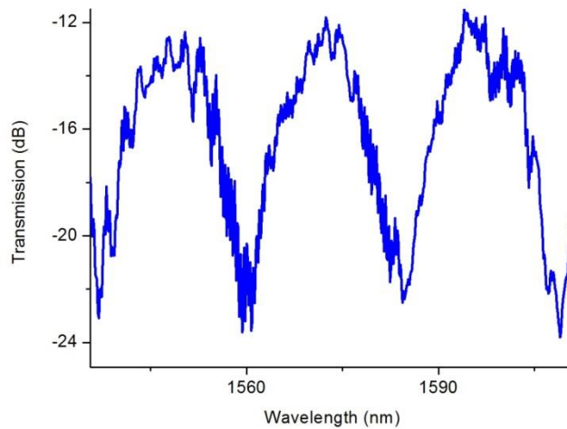
Fig. 4. Optical transmission of the asymmetric Mach-Zehnder interferometer made of Ge-rich SiGe waveguide on graded SiGe buffer
