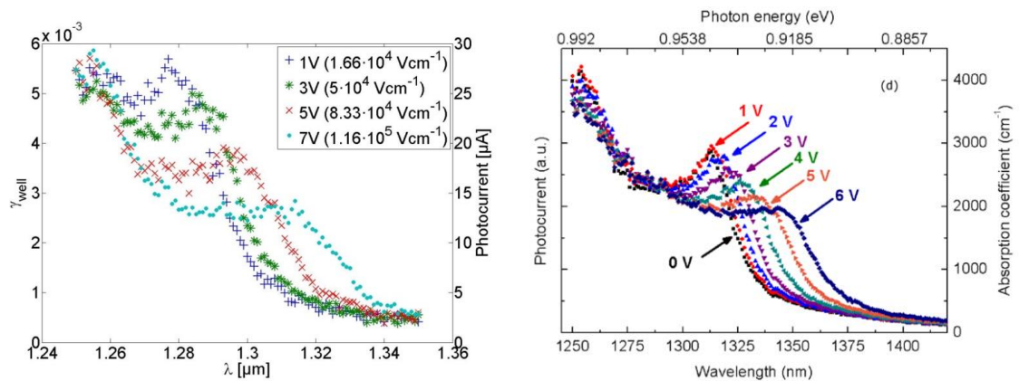
Fig. 2. QCSE in the O-band telecommunication wavelength, based on (a) strain engineering, (b) thickness engineering of the QW structures
