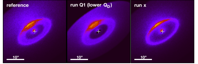
Fig. 21. Synthetic scattered light images of three of the runs: (left) the reference, (middle) Q1, and (right) x. Note that run Q1 is artificially truncated at a radial distance of 400 AU (25''). All three disks are inclined by 60 degrees with respect to the sky plane, the north-eastern part being closer to the observer.
