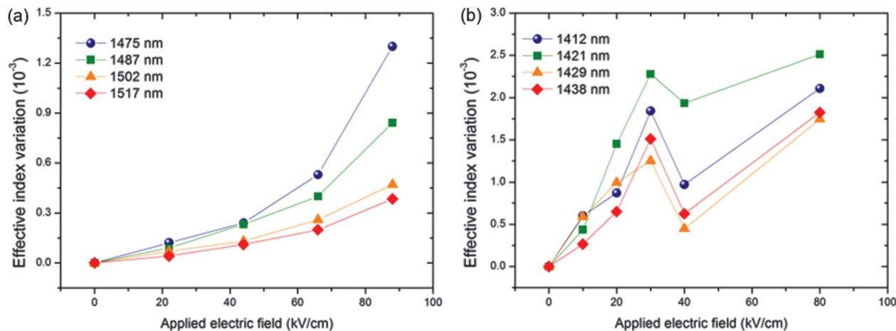
Fig. 3. Effective index variation as a function of the applied electric field at different wavelengths for sQW (a) and cQW (b).
