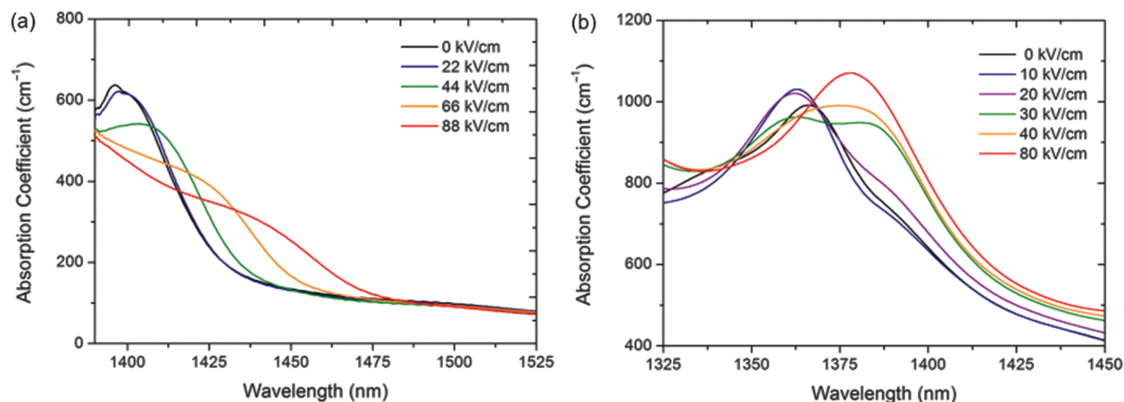
Fig. 4. Smoothed absorption spectra for different applied electric fields for sQW (a) and cQW (b).
