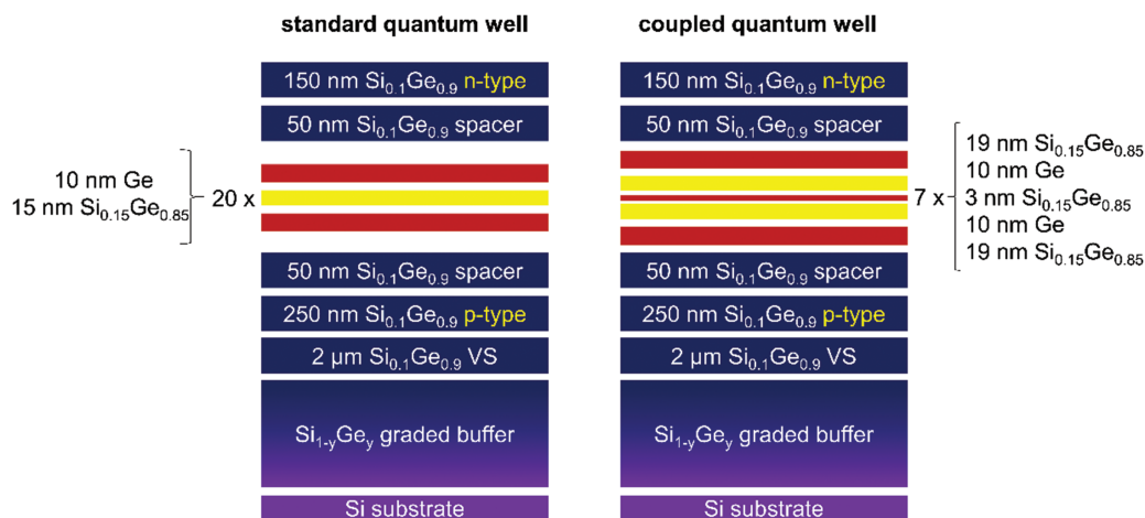
Fig. 1. Schematic of the sample with detailed growth steps.
