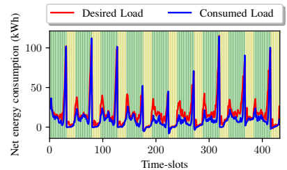
Fig. 3. Net load asked in the market versus the net load actually consumed.
