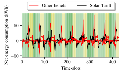
Fig. 2. All net profiles obtained by using different beliefs in one simulation with a ToU rate.
