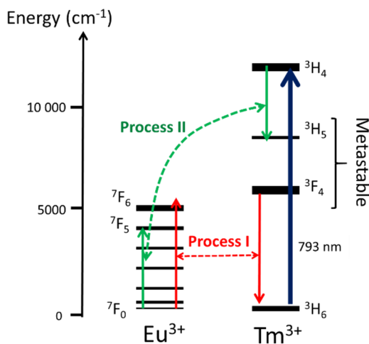
Figure 1: Energy level diagram of \text{Tm}^{3+} and \text{Eu}^{3+} in YAG and energy transfer schemes.
