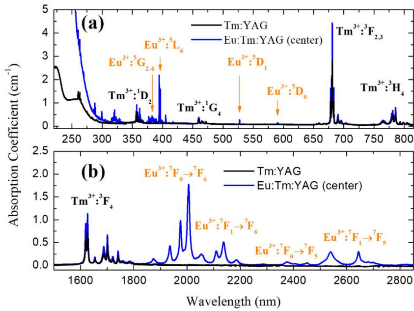
Figure 3: Blue line: Absorption spectra of Eu:Tm:YAG single crystal (center part) at room temperature in UV-visible (a) and IR region (b). Transitions of Tm^{3+} and Eu^{3+} are labeled in black and orange, respectively. Black line: The spectra of Tm:YAG single crystal are also shown for comparison.
