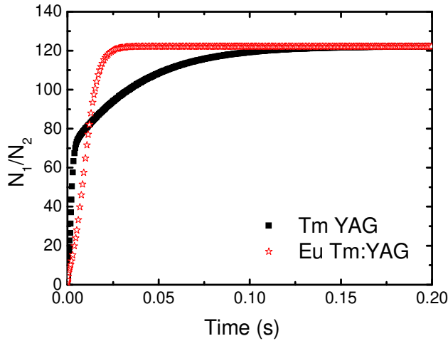
Figure7: Variation of the hyperfine population ratio ( N_1/N_2 ) with time simulated by numerical calculation. Squares and stars represent the simulation for Tm:YAG and Tm,Eu:YAG respectively.
