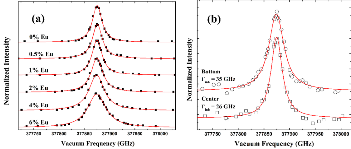
Figure 9: (a) Excitation spectra of Tm^{3+} : ^3H_6 \rightarrow ^3H_4 transition of the ceramics at 10 K by probing the 1.54 \mu m transition. Tm^{3+} concentration in all these samples is 0.5%. (b) Inhomogeneous absorption line of the Tm^{3+} : ^3H_6 \rightarrow ^3F_4 transition in Eu:Tm:YAG single crystal samples at 10 K.
