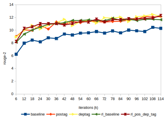
Figure 3: Evolution on test set during training
