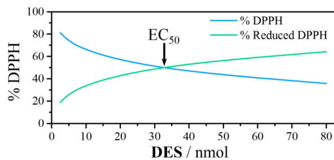
Fig. 5. Antiradical activity determination via DPPH assay, the EC_{50} is provided by the crossing point of % DPPH (blue) and % reduced DPPH (green), which occurs at 32.7 nmol.
