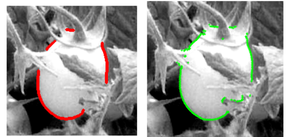
Figure 9: Two different set of points \mathbf{P}_h and \mathbf{P}'_h .
