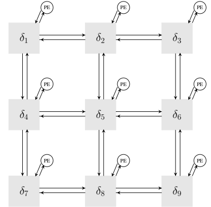
Fig. 1: 2D-Mesh NoC Architecture
