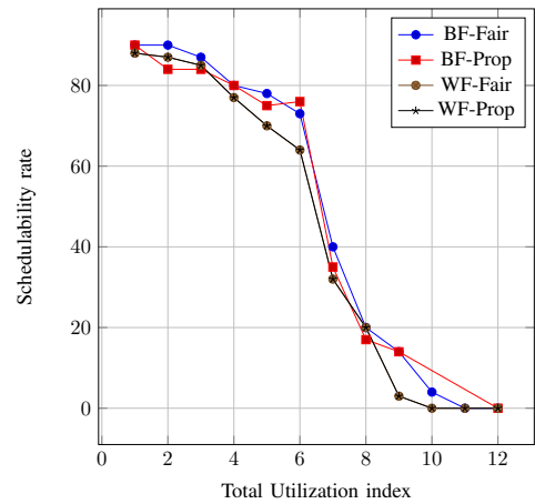
Fig. 4: Heuristics schedulability rate by tasks utilization rate
