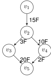
Fig. 2: An example of a dag task
