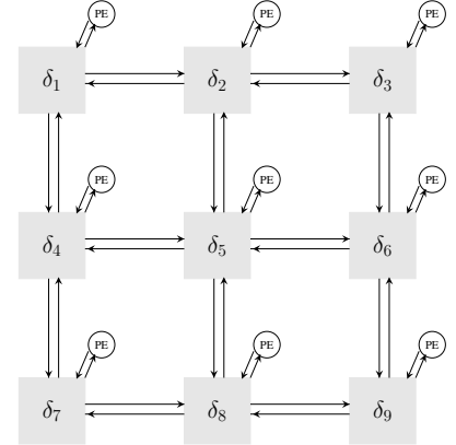
Fig. 1: 2D-Mesh NoC Architecture
