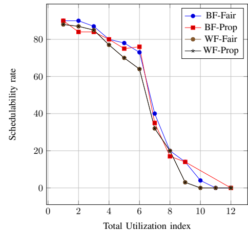
Fig. 4: Heuristics schedulability rate by tasks utilization rate
