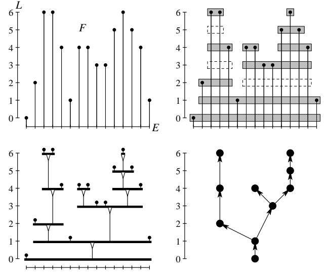
Fig. 14 Here E is a one-dimensional digital set of 15 points, and the connection \mathcal{C} corresponds to the adjacency relation between consecutive points. We take L = \{0, 1, 2, 3, 4, 5, 6\} . Top left: the function F . Top right: we show in grey the sets C \times \{h(C)\} for all C \in \text{Comp}(F) ; when C \in \text{PC}^C(X_t(F)) for t < h(C) , the set C \times \{t\} is shown dashed. Bottom left: when the altitude decreases from \top to \perp , a point p enters at altitude F(p) the component C such that p \in C and h(C) = F(p) ; then C gets included in the component C' of highest altitude that strictly contains C . We obtain a dendrogram drawn upside down. Bottom right: each component becomes a node of the max-tree, with parent-child directed edges corresponding to the covering relation in the dendrogram.
