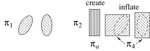
Fig. 8 Illustration of Theorem 14: from \pi_1 \boxsubseteq \pi_2 we get \pi_1 \subseteq \pi_1 \cup \pi_a \trianglelefteq \pi_2 and \pi_1 \trianglelefteq \pi_4 \subseteq \pi_2 .
