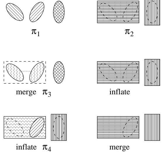
Fig. 7 Illustration of Theorem 12: from \pi_1 \boxtimes \pi_2 (top) we get \pi_1 \sqsubseteq \pi_3 \trianglelefteq \pi_2 (middle) and \pi_1 \trianglelefteq \pi_4 \sqsubseteq \pi_2 (bottom).
