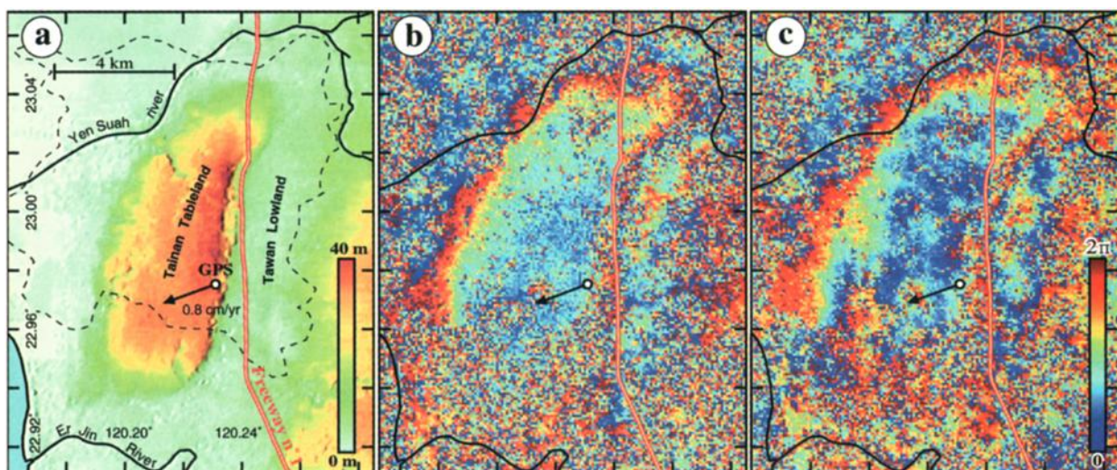
Figure 2. a) Topography and shaded relief of the Tainan area. b) Interferogram A-E (701 days, h_a = -1141 m). c) Interferogram B-D (665 days, h_a = 57 m). Both independent interferograms AE and BD having different ambiguity altitude values show one fringe which well agrees with the outline of the tableland. The fringe indicates an uplift of the Tainan Tableland in the 2 years time interval. The noisy aspect of interferogram BD is due to atmospheric artefacts on image D. Hydrography and coastline are in black thick line, the white circle with arrow represents I004 GPS station and its displacement. Dashed line represents the outline of the urban area of Tainan.
