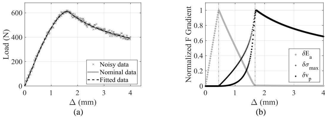
Figure 5: (a) Synthetic measurements data with its optimisation result; (b) Normalized sensitivity functions for the load displacement mechanical response
