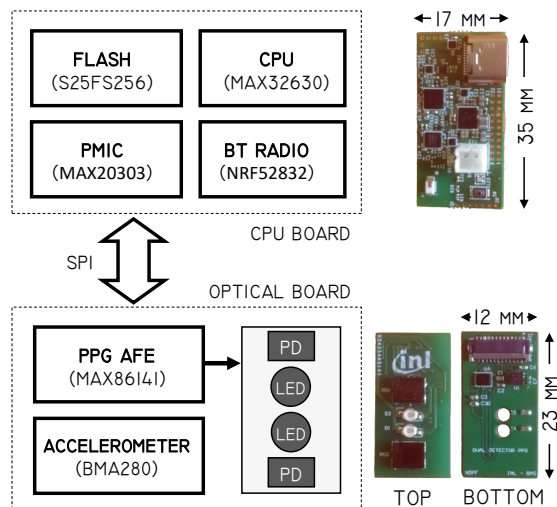
Figure 1: Acquisition system architecture.
