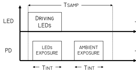
Figure 2: PPG AFE Acquisition Timing.
