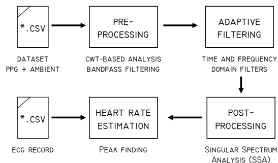
Figure 12: Signal processing toolchain architecture.
