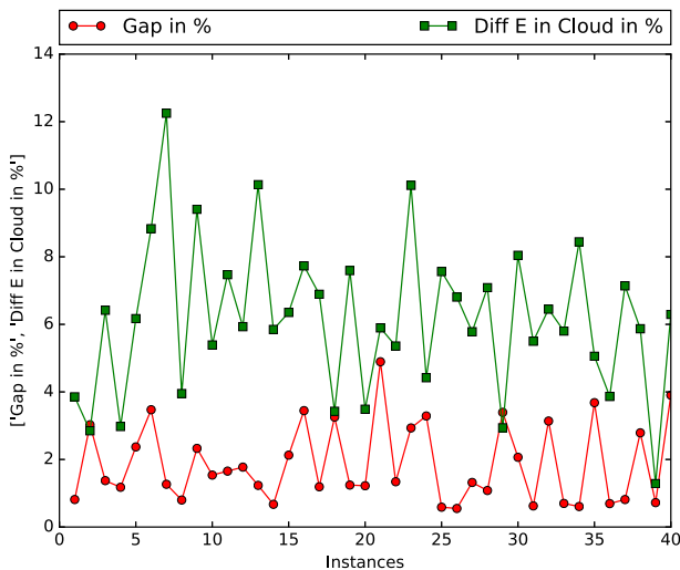
Fig. 11 Gurobi gap and the difference of energy consumption between optimizing energy and optimizing makespan in the Cloud setting
