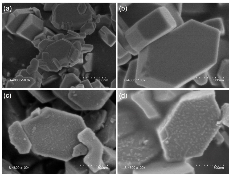
Figure 2. SEM images of a-b) the pristine LCP, b) LCP-F1 and c) LCP-F2
