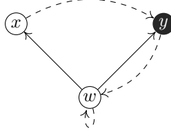
Figure 2: Example of an \text{ITL}^e model \mathfrak{M} = (W, \preceq, S, V) , where \preceq is the reflexive and transitive closure of the relation indicated by the solid arrows, S is the relation indicated by the dashed arrows, and a black dot indicates that the variable p is true, so that we only have p \in V(y) . Then, the reader may verify that \mathfrak{M}, x \models \text{Op} but \mathfrak{M}, x \not\models p , while \mathfrak{M}, y \models p but \mathfrak{M}, y \not\models \text{Op} . From this it follows that \mathfrak{M}, w \not\models (\text{Op} \rightarrow p) \vee (p \rightarrow \text{Op}) .
