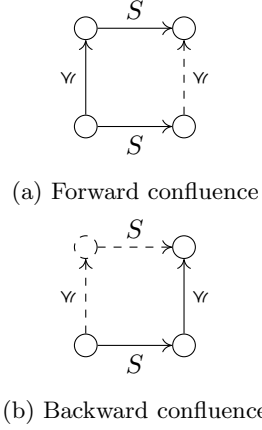
Figure 1: On a dynamic poset the above diagrams can always be completed if S is forward or backward confluent, respectively. Posets with both properties are persistent .
