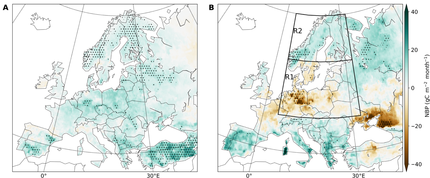
Fig. 2. Anomalies of \text{CO}_2 fluxes during spring and summer 2018. Spatial patterns of NBP anomalies (reference period 1979–2018) during (A) spring (MAM) and (B) summer (JJA) 2018 estimated by the MMEM of 11 DGVMs. A positive (negative) value indicates higher (lower) net \text{CO}_2 uptake than the 40-year average. The color map shows the multimodel ensemble mean anomalies, and the stippling indicates those regions with extremely low (rank 40th) or extremely high (rank 1st) values over the reference period.
