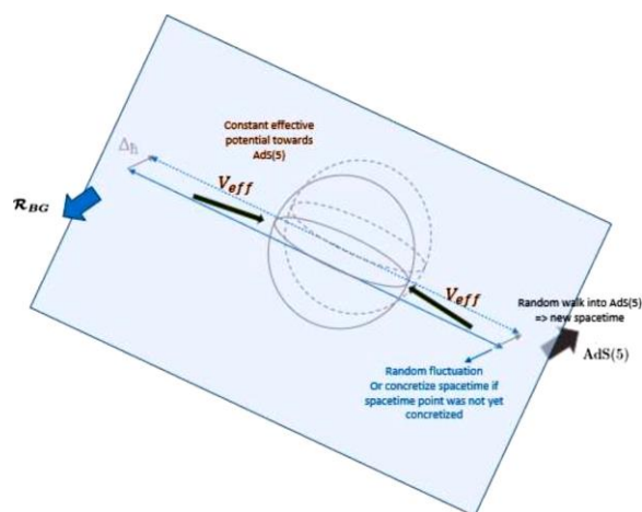
Figure 15: Fluctuations of the position of the entangled particles, result into the attractive effective potential to point towards the tangent dual AdS(5) space and produce a (constant) force to grow spacetime and hence accelerate expansion. Fluctuations within spacetime only introduce torsion, or fluctuations in spacetime, or concretize not yet existing spacetime as constant rate processes (lattice points never occupied vs. in the first case where new lattice points are created in an accelerated way). The figure illustrates symbolically the 4-D spacetime.
