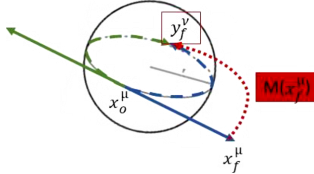
Figure 2: It illustrates a fold F (for: x_0^\mu, f ) at time f for two EPR entangled particles. The mapping is also illustrated for the segment [x_0^\mu, x_f^\mu] to the equator going from x_0^\mu = x_f^v to y_f^v = M(x_f^\mu) , for the closest particle (part1). A P-symmetric (i.e., a reflection) mapping exists for the symmetric segments associated to the other particle part2. Any entity meeting [x_0^\mu, x_f^\mu (part 1)] \cup [x_0^\mu, x_f^\mu (part 2)] encounters the support domain of the mapping \mathcal{D}(M) (the figure is for \mathcal{D}_{tear}(M) ). This is one possible fold associated to x_0^\mu(f) . As the time, here noted f , changes, the fold also evolves to continue to match this figure: the fold grows proportionally to x_f^\mu itself proportional to the elapsed time (if we assume constant momentum for each particle). With hard-partitioned fold instances per particle, interactions between the two entangled particles are allowed only at y_f^v = M(x_t^\mu) , besides the entry point. The fold grows as the particles move apart.
