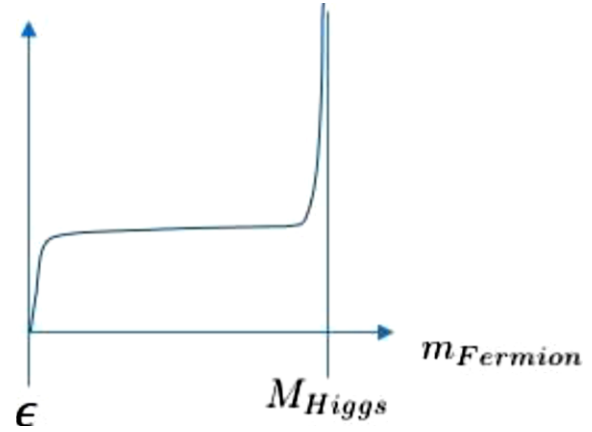
Figure 13: Plot of the value of equation (28) (vertical axis) that shows the three regions of Fermion mass in a family corresponding to three and only three generations per family: one with minimum mass, one with a mass close to the mass of the Higgs boson and one somewhere in between. It relies on estimating the impact on K_1 and K_2 and, in particular, the expectation that their value are larger when the mass matches the mass of the Higgs Boson. Only these three regimes are differentiated; any other kind of fermion in a family would have the same mass as one of these three and be hard to distinguish.
