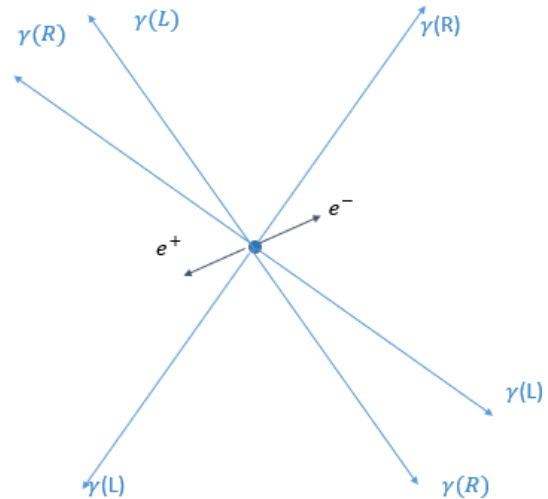
Figure 5: Real particles are surrounded by virtual particles that are created EPR entangled and initiate the multi-folds activations. They result into gravity-like effects for particles crossing the support domain of the mappings for these entangled virtual particles. The effect is isotropic and also involves massive virtual particles at very small scales with similar effects as massless effects, at these scales. Multi-folds live outside spacetime in a tangent dual space.
