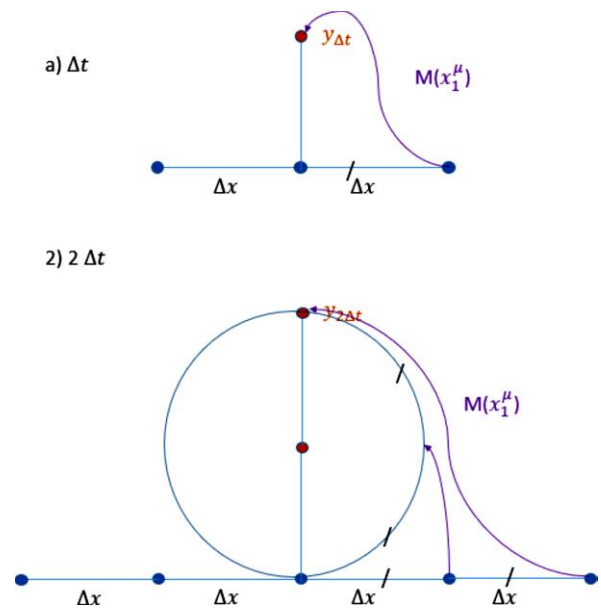
Figure 14: Growth of entangled spacetime by random walk or at inflation has spacetime points entangled locally at least for a while. The growth in spacetime matches the growth of the multi-folds. These deltas in spacetime and in folds are the quanta of the multi-fold mechanism (growth of the multi-folds), on in each fold, per (random) time click. They match the space-time growth or changes in \mathcal{R}_{BG} encountered in conventional quantization of gravity/ GR and of gravity as a result. These are the gravitons in U_{MF} : in our model, they live outside the spacetime \mathcal{R}_{BG} but match the perturbation and growth in \mathcal{R}_{BG} .
