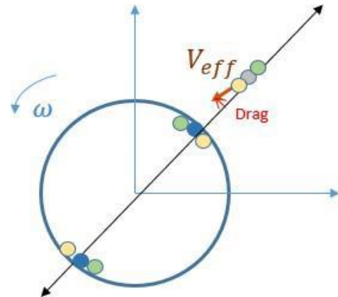
Figure 10: In the rotating frame the integration from +\infty , the virtual particles contribute attraction that has a tangential component in an external inertial frame. The particles contributing to a line are symbolically shown. The contribution of the particle coming from the direction opposite to the rotation dominates. Close enough to the rotating body, it brings a V_{eff} contribution in the direction of rotation.
