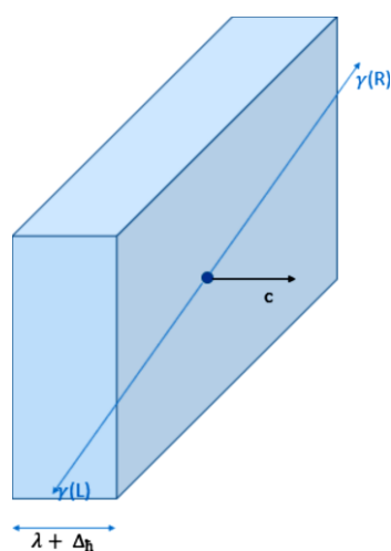
Figure 6: When considering massless particles, only massless virtual particles are involved within the plane orthogonal to the direction of propagation of the massless particle. The effect is rather a parallelepiped because of the need to model a massless particle on at least the width of a wavelength (and the associated uncertainty principle). Massive effects essentially do not appear as massive virtual particles are too hard to generate up to the uncertainty principle allowances. As no reference frame can follow the particle. From a different reference frame, it will appear as a wake trailing the massless particle.
