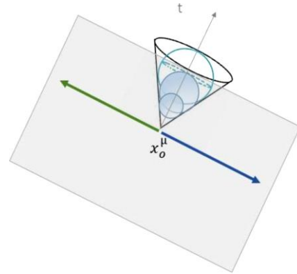
Figure 8: Cones of folds built by wrapping the spheres evolving with t tangent to U_{MF} .
