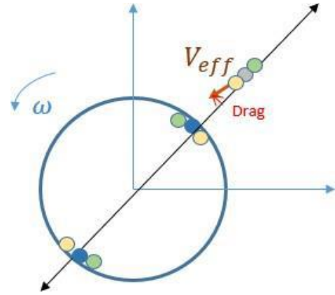
Figure 10: In the rotating frame the integration from +\infty , the virtual particles contribute attraction that has a tangential component in an external inertial frame. The particles contributing to a line are symbolically shown. The contribution of the particle coming from the direction opposite to the rotation dominates. Close enough to the rotating body, it brings a V_{eff} contribution in the direction of rotation.
