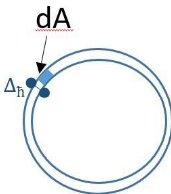
Figure 12: All the gravity effects of the black hole are captured in a shell of constant depth and a surface A . These represent all the gravity or spacetime degrees of freedom of the black hole as they (and only these points) generate what is perceived outside the black hole. The Gauss theorem works with \Sigma (no light sheets needed) as all trapped particles (real or virtual) behave massively when trying to exit: the massless multi-fold pattern can be ignored.
