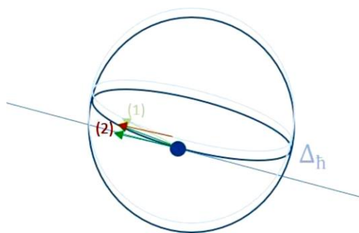
Figure 7: When uncertainty moves the source or an emitted entangled virtual particle, it shifts the fold, or the fold is then shifted back or tilted, in order to support later mapping to the same exit point and depending on the uncertainty changes. Between the oscillations, the momentum of the virtual particle entering the fold (path on the fold) is oscillating back and forth between (1) and (2) resulting into a spiral move.
