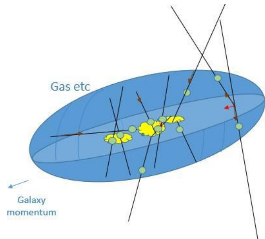
Figure 16: Entanglement from matter or between emitted entangled pairs of particles creates impressions of attraction towards the galaxy or halos of the galaxies. If not, enough matter is kept entangled in or towards galaxy (or if not, enough halo exists to capture entanglement with the center, the effect may decrease or become negligible).
