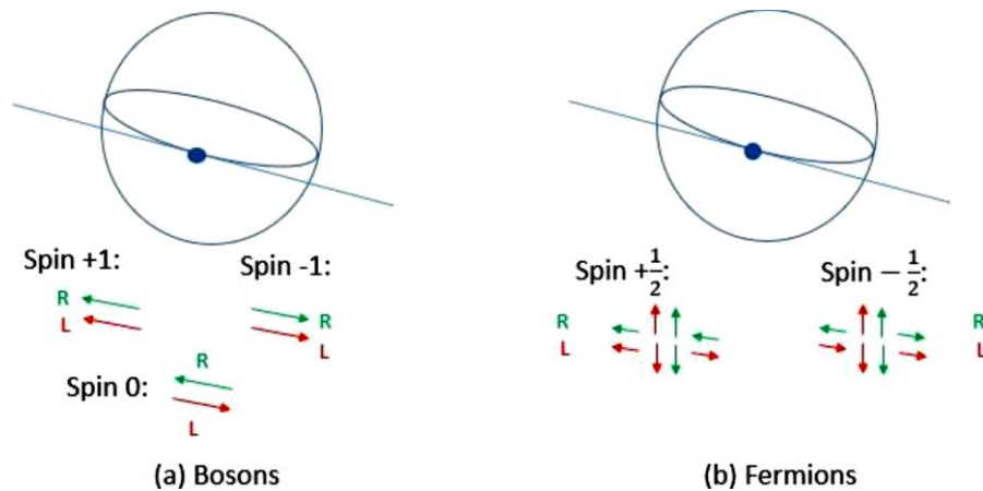
Figure 9: It illustrates possible patterns of distribution of how entangled virtual particles could enter paths in the activated folds to provide different spins (by rotating the spacetime around the folds). The virtual particles are dominated by virtual photons with two possible polarities ( R and L ). Entries can be along the grand circle along the direction of propagation of the virtual particles or orthogonal (to have independent contributions). With a not yet quantized model for gravity, this can be in any direction as virtual particles are emitted in an isotropic manner and the criteria for one pattern to another are not explained other than for symmetries of (a) 360^\circ for bosons vs. (b) 720^\circ for fermions, where entry patterns and polarizations of the photons have to be considered.
