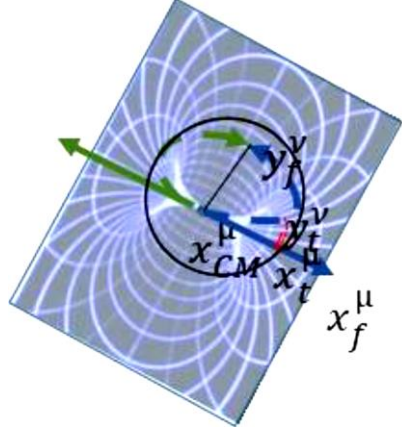
Figure 4: The contribution of \mathcal{P}I_{B_{active}(for: x_{CM(t)}^\mu, t)}(S, \psi)|_{(part(t) \in D(M))} includes integration over 2\pi . The bundles of fold are sets of tori. Here, we assume: D(M) = [x_{CM(t)}^\mu, x_t^\mu(part_1)] \cup [x_{CM(t)}^\mu, x_t^\mu(part_2)] .
