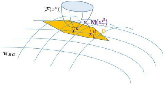
Figure 1: Illustration of a generic fold \mathcal{R}_F(x^\mu) activated around a point x^\mu with a mapping M that indicates how other points in the support domain \mathcal{D} of M appear on \mathcal{R}_F(x^\mu) . Paths crossing the support domain \mathcal{D} add a contribution from M(x_1^\mu) (an entry point), from where some paths are considered on \mathcal{R}_F(x^\mu) (to an exit point).
