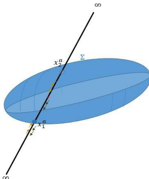
Figure 11: If a contributing point is moved between [x_1^a, x_2^a] , the gain or loss of contributing folds felt by x_1^a is compensate by the loss or gain coming from change on x_2 side. As a result, points can be moved to a more internal surface \Sigma' the effect felt on \Sigma . When the surface is not static, or we consider massless sources, we need to revert to the lights sheets built on \Sigma , as in [518].
