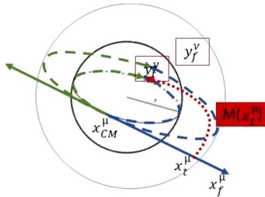
Figure 3: The contribution of \mathcal{PI}_{\mathcal{B}_{active}(for: x_{CM}^\mu, t)}(S, \psi)|_{(part(t) \in \mathcal{D}(M))} includes integration over r . Here, we assume:
