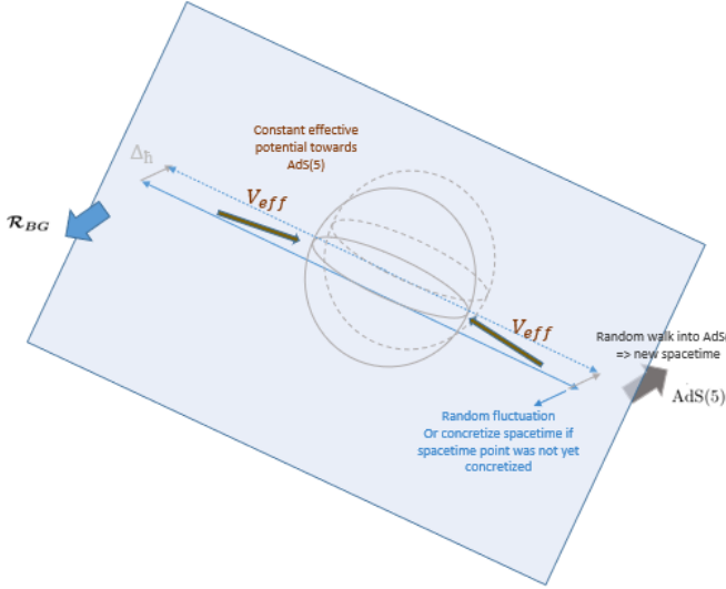
Figure 15: Fluctuations of the position of the entangled particles, result into the attractive effective potential to point towards the tangent AdS(5) space and produce a (constant) force to grow spacetime and hence accelerate expansion. Fluctuation within spacetime only introduce torsion or fluctuation in spacetime or concretize not yet existing spacetime as constant rate process (lattice points never occupied vs. in the first case where new lattice points are created in an accelerated way). The figure illustrates symbolically the 4-D spacetime.
