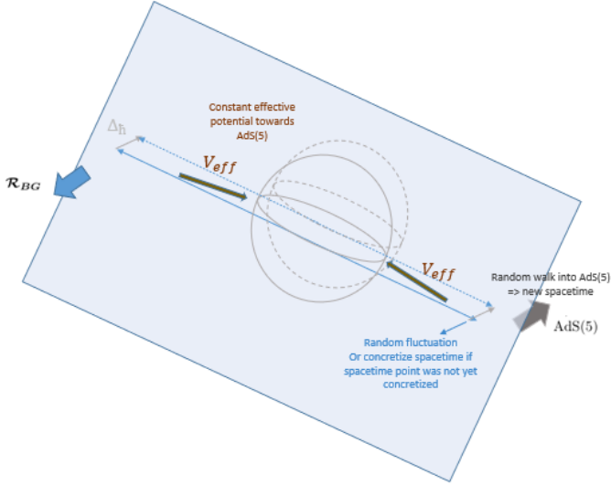
Figure 15: Fluctuations of the position of the entangled particles, result into the attractive effective potential to point towards the tangent AdS(5) space and produce a (constant) force to grow spacetime and hence accelerate expansion. Fluctuation within spacetime only introduce torsion or fluctuation in spacetime or concretize not yet existing spacetime as constant rate process (lattice points never occupied vs. in the first case where new lattice points are created in an accelerated way). The figure illustrates symbolically the 4-D spacetime.
