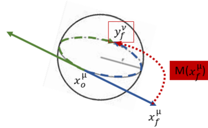
Figure 2: It illustrates a fold \mathcal{F}(for : x_0^\mu, f) at time f for two EPR entangled particles. The mapping is also illustrated for the segment [x_0^\mu, x_f^\mu] to the equator going from x_0^\mu = y_0^\nu to y_f^\nu = M(x_f^\mu) , for the closest particle ( part_1 ). A P -symmetric (i.e. a reflection) mapping exists for the symmetric segments associated to the other particle part_2 . Any entity meeting [x_0^\mu, x_f^\mu(part_1)] \cup [x_0^\mu, x_f^\mu(part_2)] encounters the support domain of the mapping \mathcal{D}(M) (the figure is for \mathcal{D}_{tear}(M) ). This is one possible fold associated to x_0^\mu(f) . As the time, here noted f , changes, the fold also evolves to continue to match this figure: the fold grows proportionally to x_f^\mu itself proportional to the elapsed time (if we assume constant momentum for each particle). With hard-partitioned fold instances per particle, interactions between the two entangled particles is allowed only at y_t^\nu = M(x_t^\mu) , besides the entry point.
