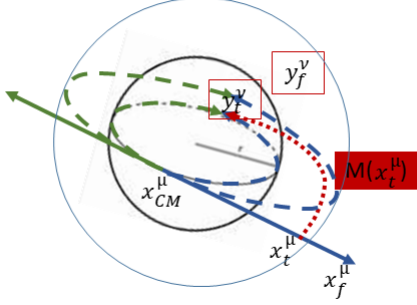
Figure 3: The contribution of \mathcal{P}\mathcal{I}_{\mathcal{B}_{activ}(for:x_{CM}^\mu,t)}(\mathcal{S},\psi)|_{part(t)\in\mathcal{D}(M)} includes integration over r . Here, we assume: \mathcal{D}(M) = [x_{CM}^\mu(t), x_t^\mu(part_1)] \cup [x_{CM}^\mu(t), x_t^\mu(part_2)] .
