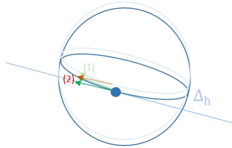
Figure 7: When uncertainty moves the source or an emitted entangled virtual particle, it shifts the fold, or the fold is then shift back or tilted, in order to support later mapping to the same exit point and depending on the uncertainty changes. Between the oscillations, the momentum of the virtual particle entering the fold (path on the fold) is oscillating back and forth between (1) and (2) resulting into a spiral move.
