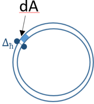
Figure 12: All the gravity effects of the black hole are captured in a shell of constant depth and a surface A . These represent all the gravity or spacetime degrees of freedom of the black hole as they (and only these points) generate what is perceived outside the black hole.
