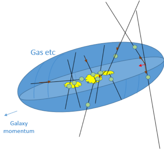
Figure 16: Entanglement from matter or between emitted entangle pairs of particles create impression of attraction towards the galaxy or halos of the galaxies. If not enough matter is kept entangled in or towards galaxy (or if not enough halo exists to capture entanglement with the center, the effect may decrease or become negligible.
