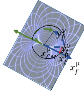
Figure 4: The contribution of \mathcal{P}\mathcal{I}_{\mathcal{B}_{activ}(for:x_{CM}^\mu,t)}(\mathcal{S},\psi)|_{part(t)\in\mathcal{D}(M)} includes integration over 2\pi . The bundles of fold are sets of tori. Here, we assume: \mathcal{D}(M) = [x_{CM}^\mu(t), x_t^\mu(part_1)] \cup [x_{CM}^\mu(t), x_t^\mu(part_2)] .
