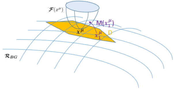
Figure 1: Illustration of a generic fold \mathcal{R}_{\mathcal{F}(x^\mu)} activated around a point x^\mu with a mapping M that indicates how other points in the support domain \mathcal{D} of M appear on \mathcal{R}_{\mathcal{F}(x^\mu)} . Paths crossing the support domain \mathcal{D} add a contribution from M(x^\mu) (an entry point), from where some paths are considered on \mathcal{R}_{\mathcal{F}(x^\mu)} (to an exit point).
