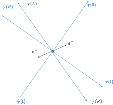
Figure 5: Real particles are surrounded by virtual particles that are created EPR entangled and initiate the multi-folds activations. They result into gravity-like effects for particles crossing the support domain of the mappings for these entangled virtual particles. The effect is isotropic and also involves massive virtual particles at very small scales with similar effects as massless effects, at these scales. Multi-folds live outside spacetime in a tangent space.
