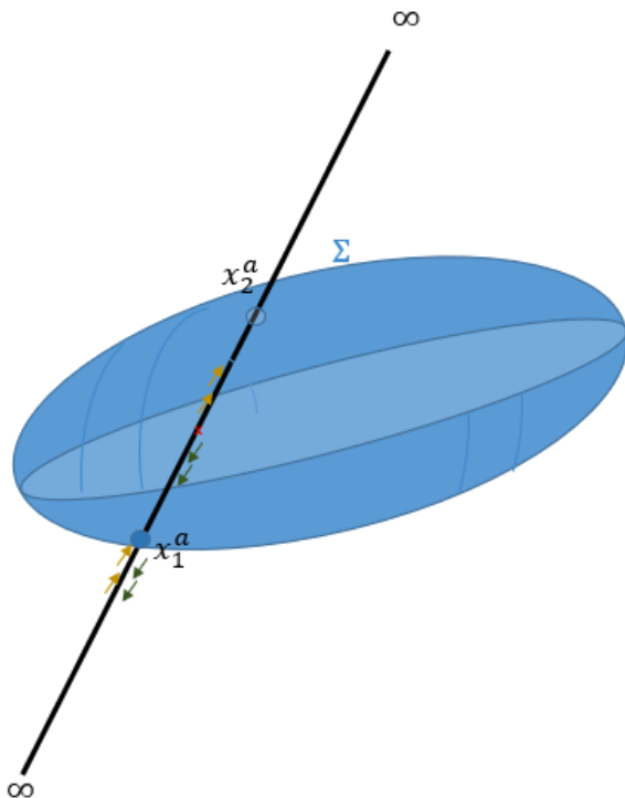
Figure 11: If a contributing point is moved between [x_1^a, x_2^a] , the gain or loss of contributing folds felt by x_1^a is compensate by the loss or gain coming from change on x_2 side. As a result, points can be moved to a more internal surface \Sigma' and not change the effect felt on \Sigma .
