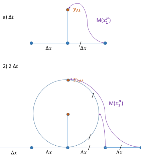
Figure 14: Growth of entangled spacetime by random walk or at inflation has spacetime points entangled locally at least for a while. The growth in spacetime matches the growth of the multi-folds. These deltas in spacetime and in folds are the quantas of the multi-fold mechanism (growth of the multi-folds), on in each fold, per (random) time click. They match the space-time growth or changes in \mathcal{R}_{BG} encountered in conventional quantization of gravity / GR and of gravity as a result. These are the gravitons in \mathcal{U}_{MF} : in our model, they live outside the spacetime \mathcal{R}_{BG} but match the perturbation and growth in \mathcal{R}_{BG} .
