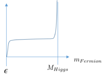
Figure 13: Plot of the value of equation (28) (vertical axis) that shows the three regions of Fermion mass in a family corresponding to three and only three generations per flavour: one with minimum mass, one with a mass close to the mass of the Higgs boson and one somewhere in between. It relies on estimating the impact on K_1 and K_2 and, in particular, the expectation that their value are larger when the mass matches the mass of the Higgs Boson. Only these three regimes are differentiated; any other kind of fermion in a family and flavour would have the same mass as one of these three and be hard to distinguish.
