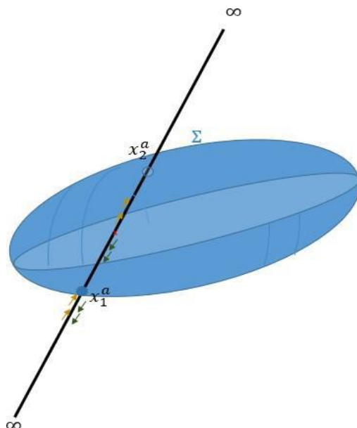
Figure 11: If a contributing point is moved between [x_1^a, x_2^a] , the gain or loss of contributing folds felt by x_1^a is compensated by the loss or gain coming from change on x_2 side. As a result, points can be moved to a more internal surface \Sigma' the effect felt on \Sigma . When the surface is not static, or we consider massless sources, we need to revert to the light sheets built on \Sigma , as in [518].
