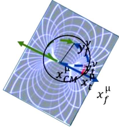
Figure 4: The contribution of \mathcal{P}I_{B_{active}(for: x_{CM}^\mu, t)}(S, \psi) |_{(part(t) \in D(M))} includes integration over 2\pi . The bundles of fold are sets of tori. Here, we assume: D(M) = [x_{CM(t)}^\mu, x_t^\mu(part_1)] \cup [x_{CM(t)}^\mu, x_t^\mu(part_2)] .
