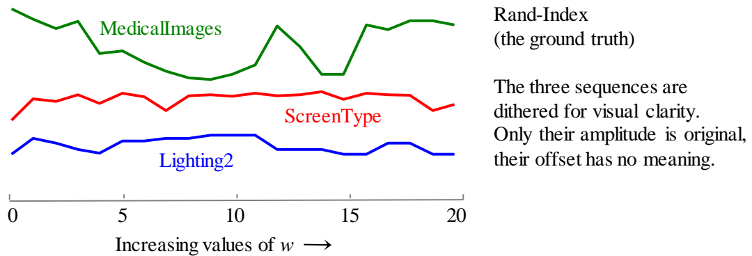
Fig. 16 The Rand-Index vs. the warping window width for three small datasets. Contrast the variability of the curves with the relatively smooth curves shown in Fig. 1.
