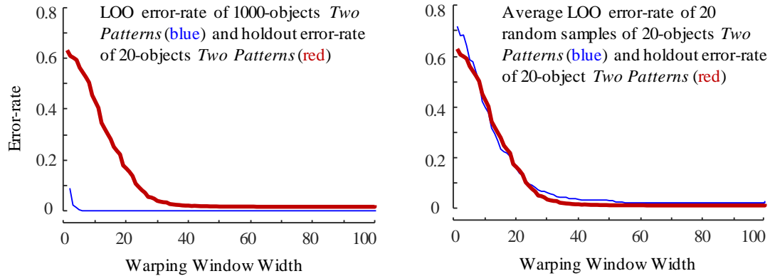
Fig. 23 left) The LOO error-rate of the Two Patterns 1000 dataset is a poor predictor of the holdout error on Two Patterns 20 . right) In contrast, the average LOO error-rate of 20 random samples of Two Patterns 20 is an excellent predictor of the holdout error on Two Patterns 20 .
