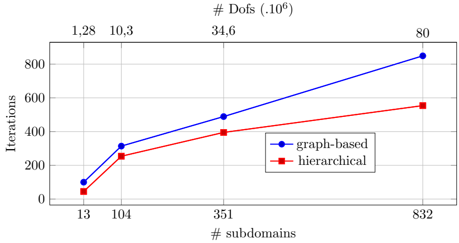
Figure 17: Convergence of the solid propellant test case for a constant size of local problems
