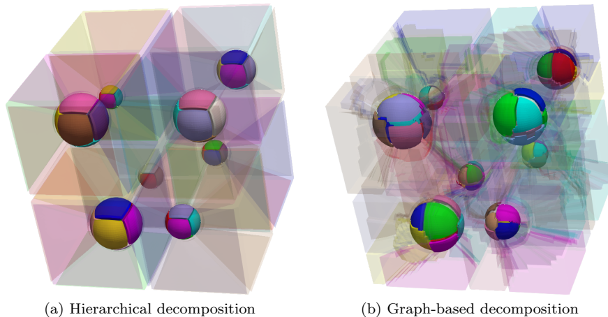
Figure 16: The solid propellant containing 2 \times 2 \times 2 inclusions, the different colors represent the different subdomains; the transparent elements represent the matrix and the others are in the inclusions
