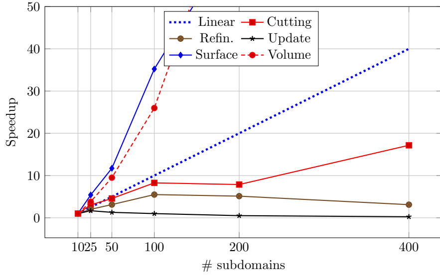
(a) Speedups of all individual timers
