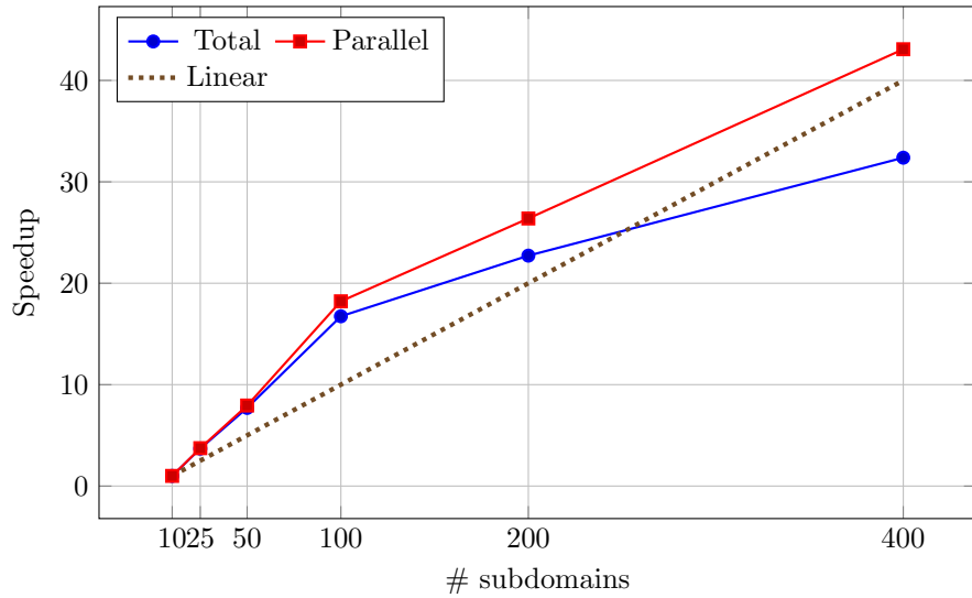
(b) Speedup of cumulated timers (Parallel={Cutting, Refin., Update, Surface, Volume}, Total={Parallel, Seq.})
