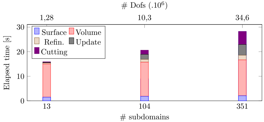
Figure 18: Time of the meshing process of the solid propellant versus the number of subdomains for a constant size of local problems
