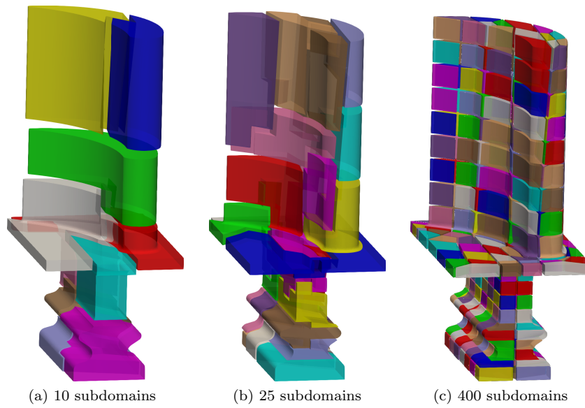
Figure 10: Hierarchical decompositions of the turbine blade
