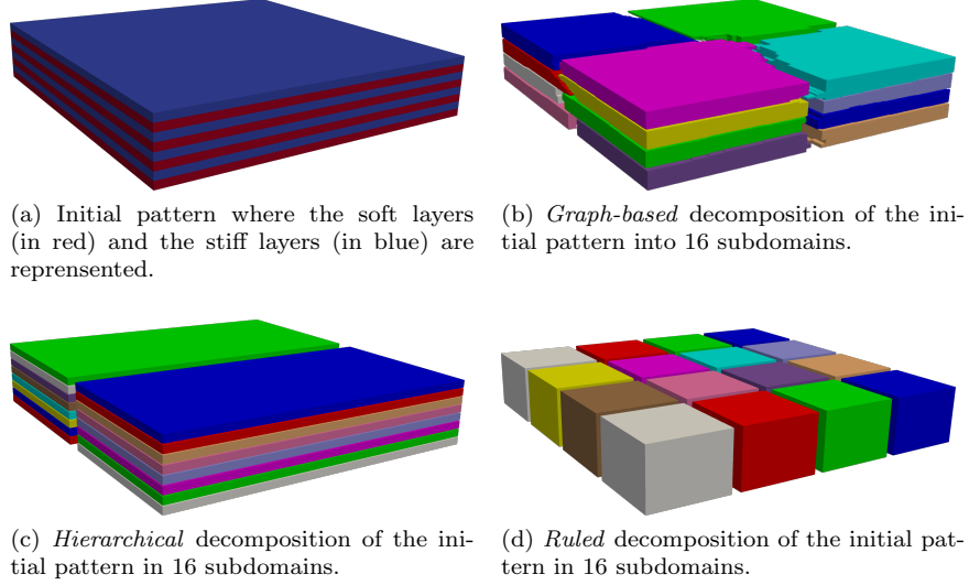
Figure 7: Initial stratified composite pattern with 545 025 nodes and 524 288 elements for different decompositions
