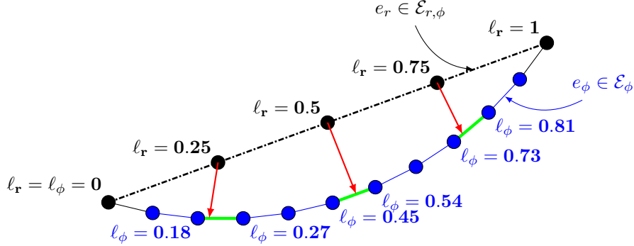
Figure 6: Projection of the edge of e_r \in \mathcal{E}_{r,\phi} (in dashed black line) on the corresponding edge e_\phi \in \mathcal{E}_\phi (in solid blue line), \ell_r and \ell_\phi are the normalized curvilinear abscissa. The green lines are the segments where the condition \ell_{r,k} \in [\ell_{\phi,K}, \ell_{\phi,K+1}] is satisfied.
