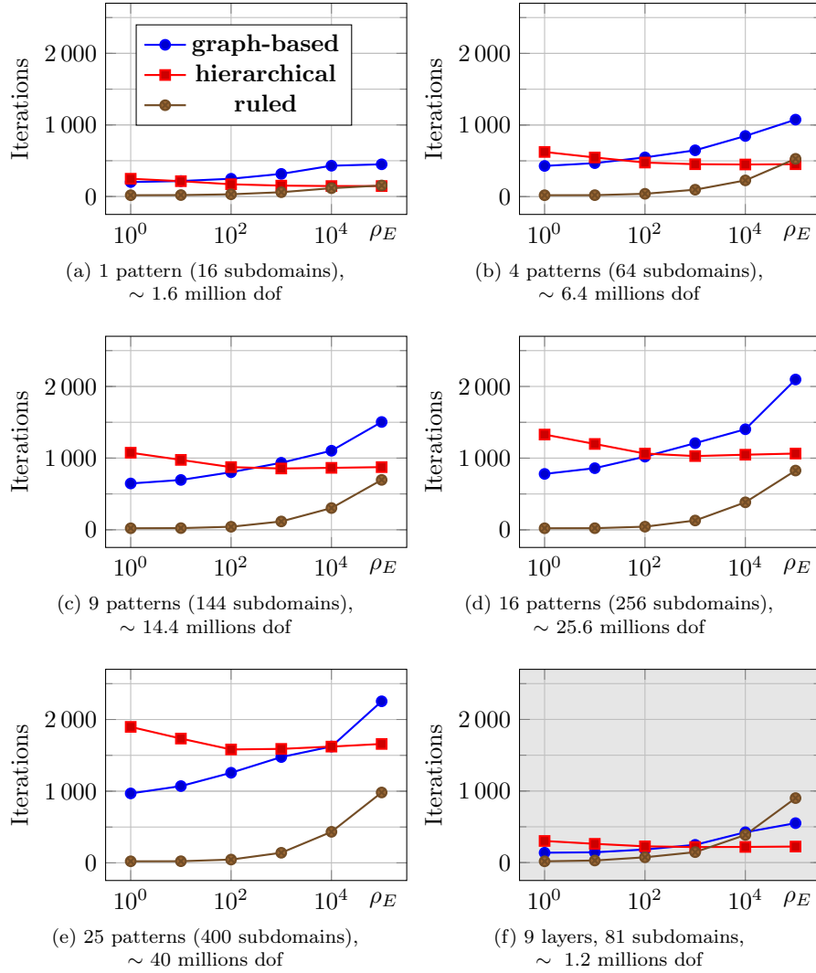
Figure 8: Stratified composite structure (a-e) 8 layers, (f) 9 layers: influence of the heterogeneity ratio \rho_E on the convergence of the FETI solver for three types of decomposition and an increasing number of subdomains.
