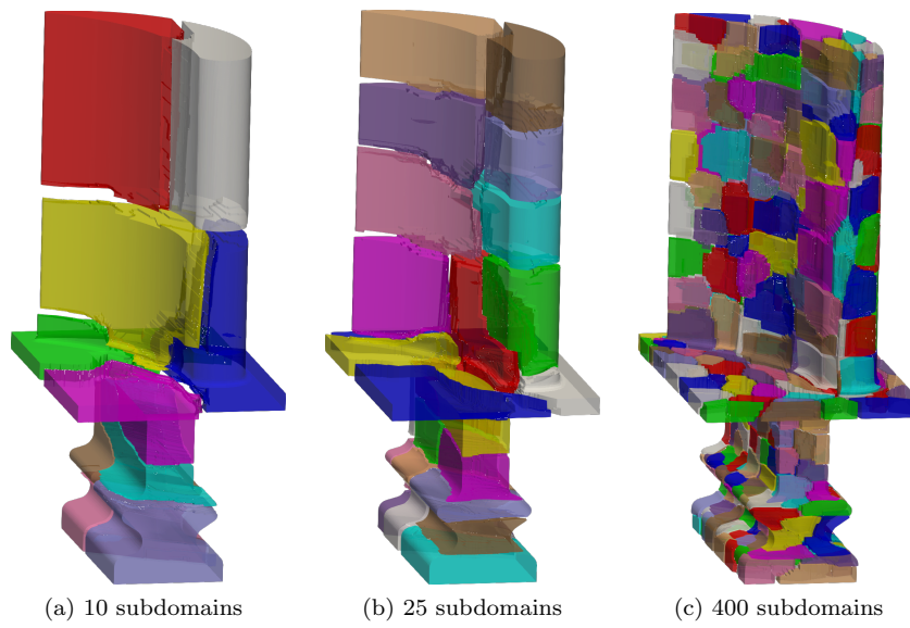
Figure 11: Graph-based decompositions of the turbine blade
