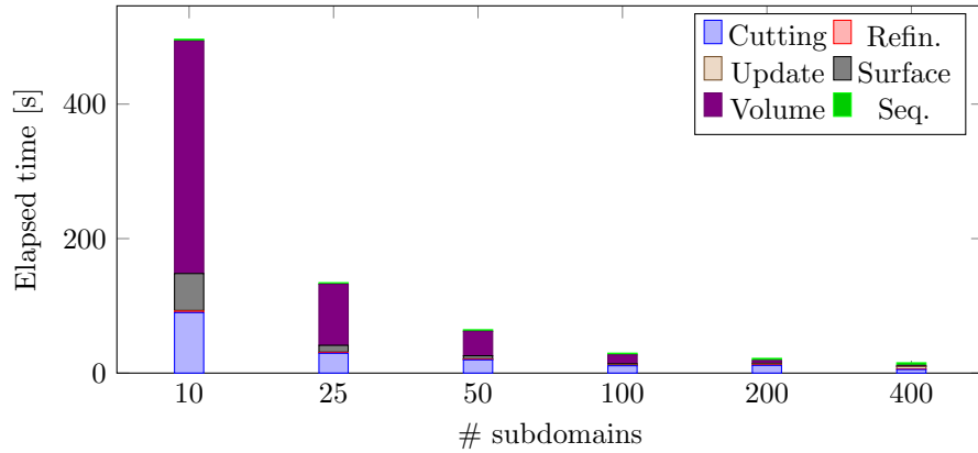
Figure 12: Elapsed time of the meshing process versus the number of subdomains for a constant size of the global problem
