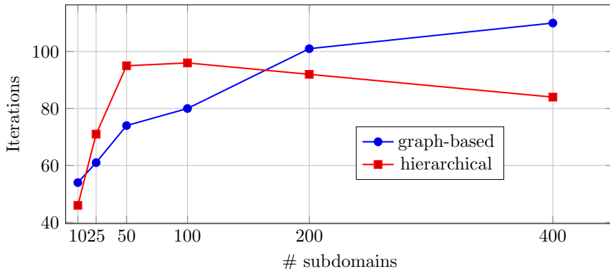
Figure 15: Number of iterations of the FETI method with a relative convergence ratio of 10^{-6} for the turbine blade case for increasing number of subdomains.
