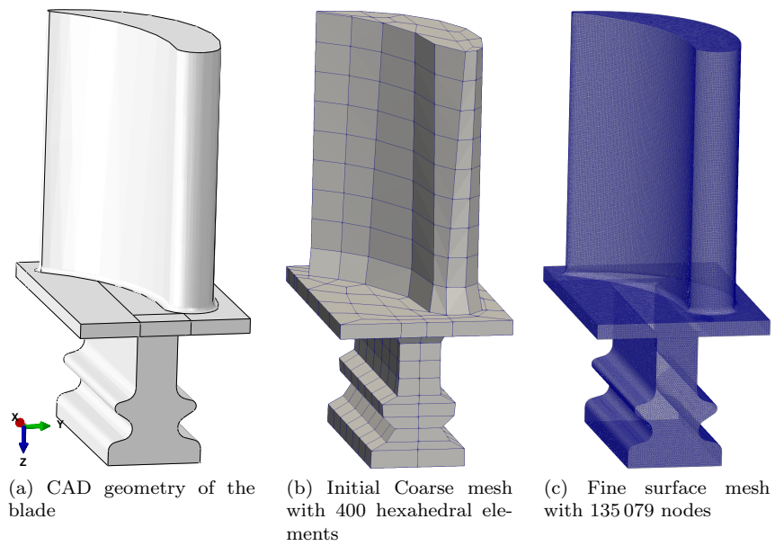
Figure 9: Initial data for the method
