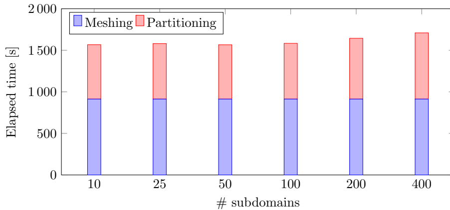
Figure 13: Elapsed time of the sequential meshing and partitioning of the blade with approximately 1.6M of nodes
