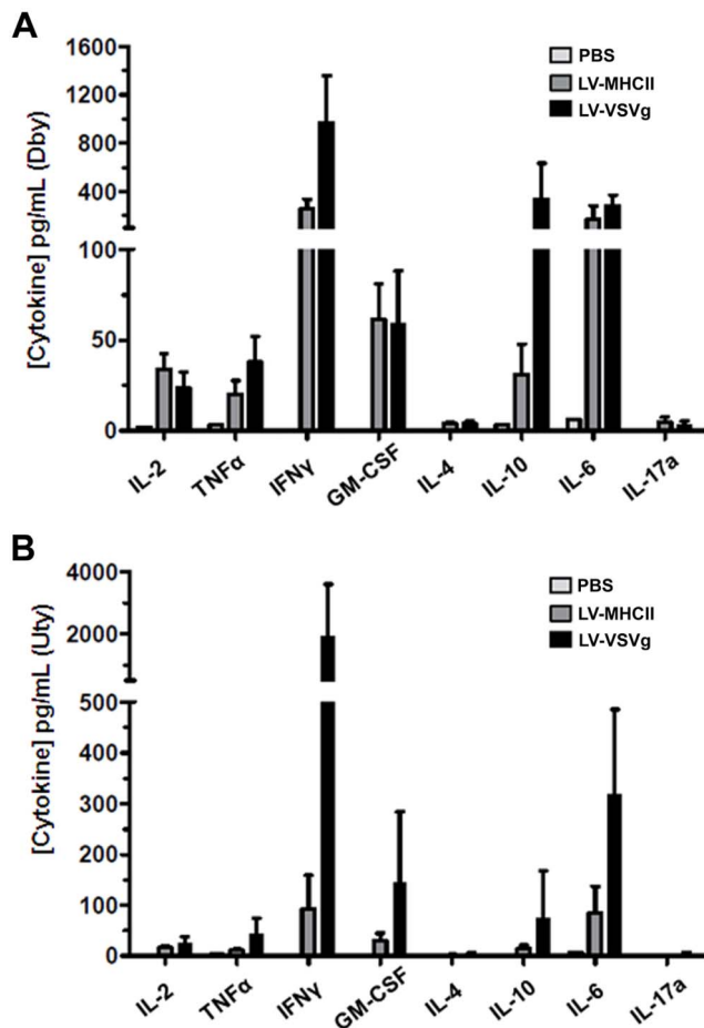
Figure 3. Cytokines secreted following immunization. C57Bl/6 female mice were injected IV with PBS, 50 ng RT of LV-VSVg or LV-MHCII vectors. 7 days later, spleen cells of these mice were harvested and assayed for IL-2, IL-4, IL-6, IL-10, IL-17A, IFN- \gamma , TNF- \alpha and GM-CSF secretion after a 48 hour stimulation ex vivo with Dby (A) or Uty (B) using the cytokine bead array (n = 5 mice per group). Data and assay limits of detection are displayed in Table 2. doi:10.1371/journal.pone.0101644.g003
